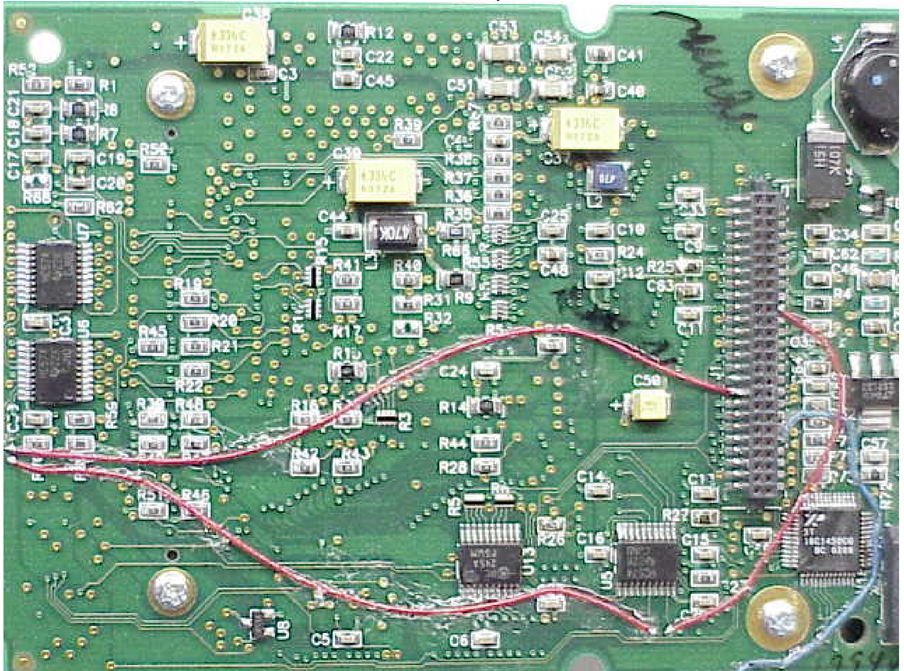
DOS Board Secondary Side
