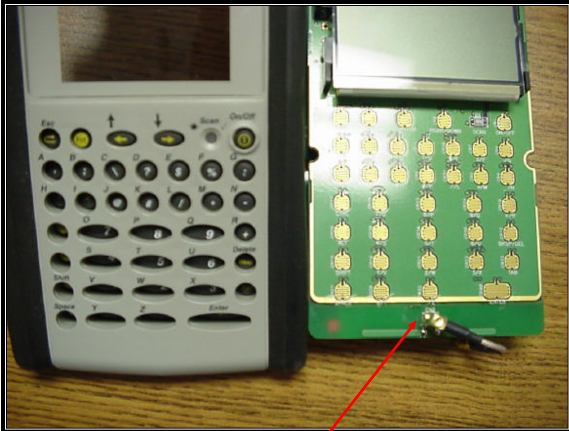
PHOTOGRAPH 13: LOCATION OF ANTENNA RELATIVE TO THE KEYPAD, ON EDGE OF THE PCB
