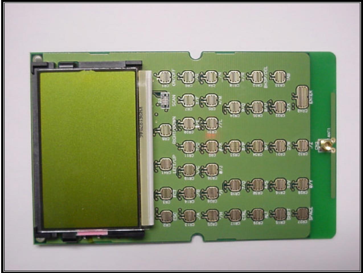
PHOTOGRAPH 18: TOP OF UPPER PCB WITH ANTENNA CONNECTOR AND TRACE
