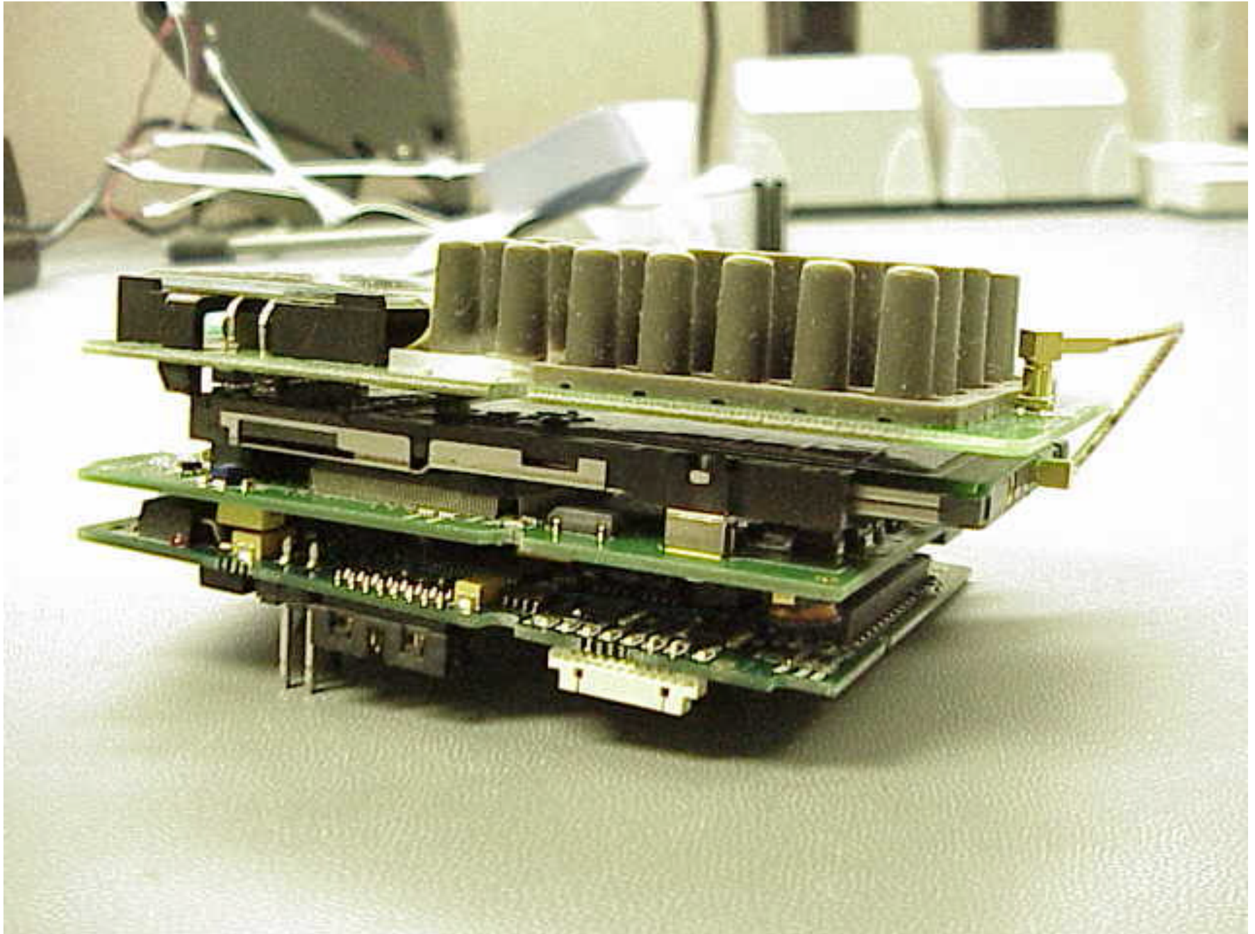
Board stack
