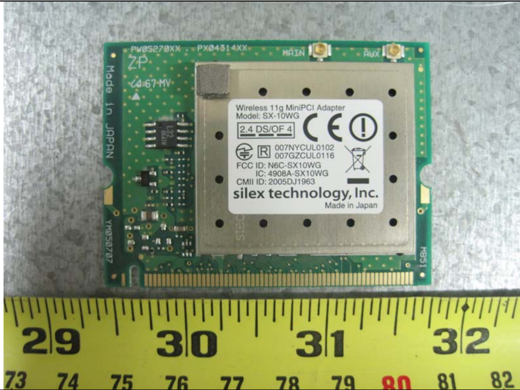
EUT (9906): RF Module PCBA Component View
