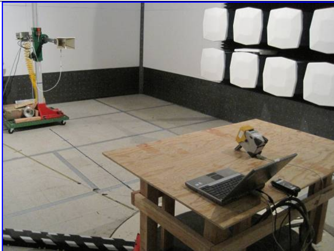
Host: 9460 Radiated Emission Test Setup – Rear View
