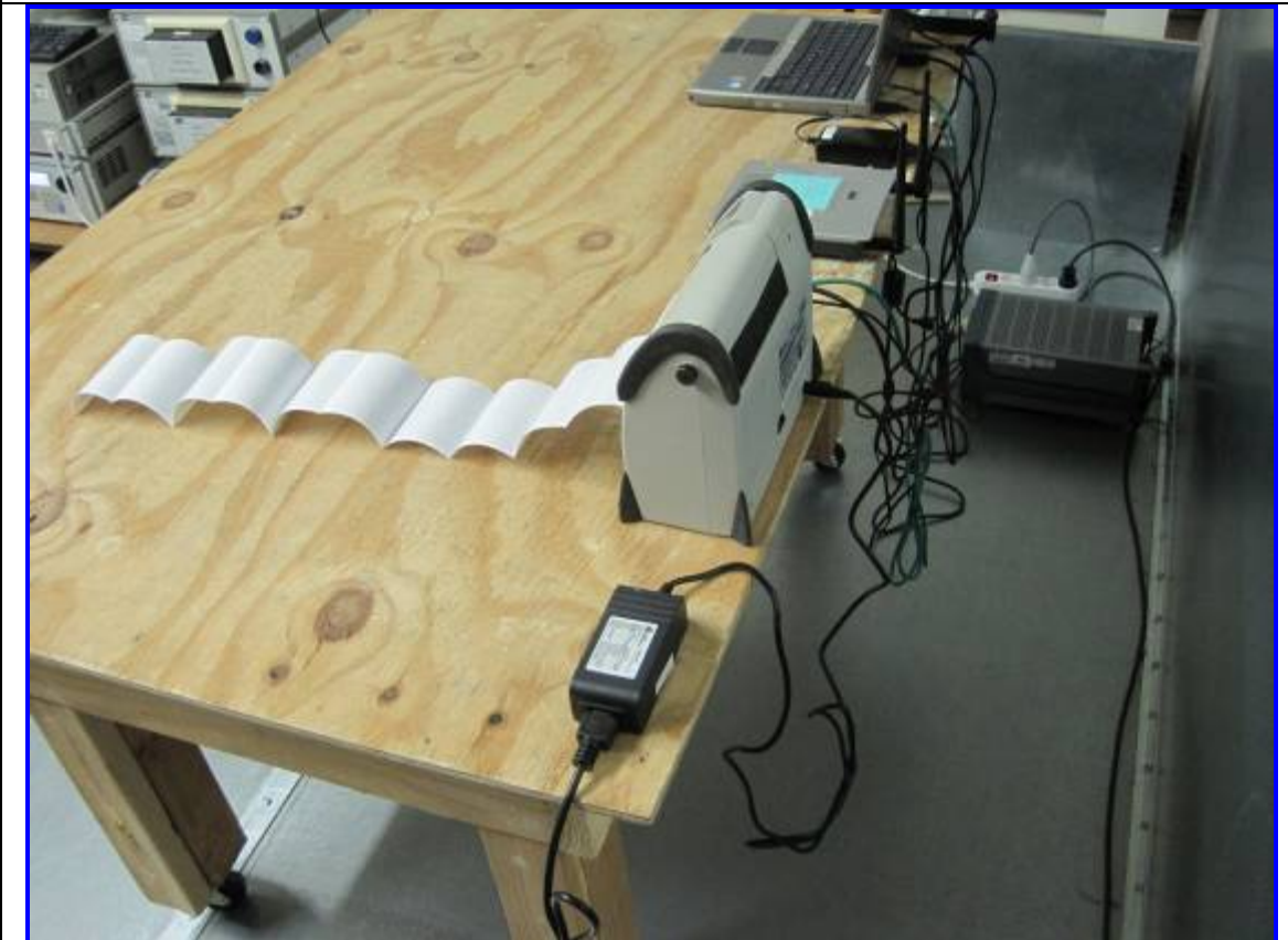
Host: 9493 Conducted Emission Test Setup – Rear View
