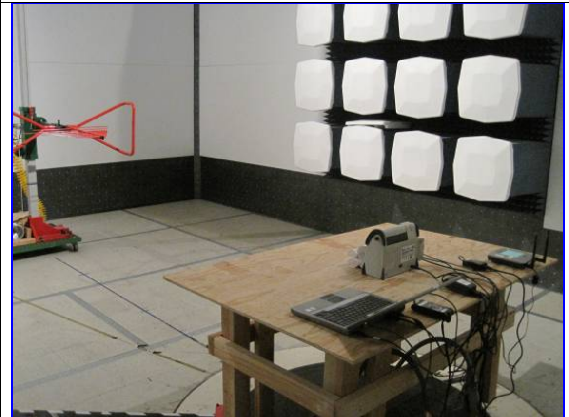
Host: 9493 Radiated Emission Test Setup – Rear View
