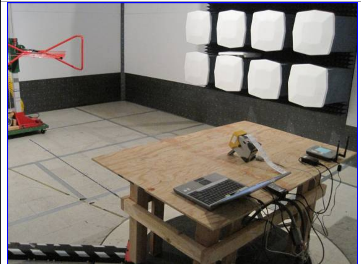
Host: 9460 Radiated Emission Test Setup – Rear View
