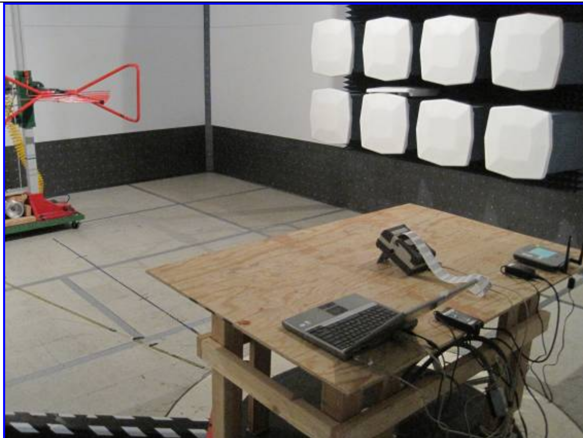
Host: 9433 Radiated Emission Test Setup – Rear View
