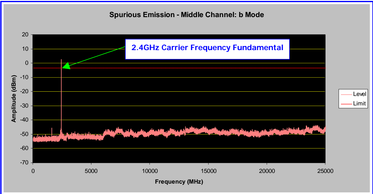
Middle Channel (802.11b)
