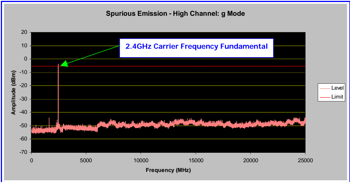
High Channel (802.11g)
