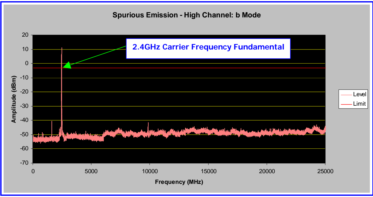
High Channel (802.11b)
