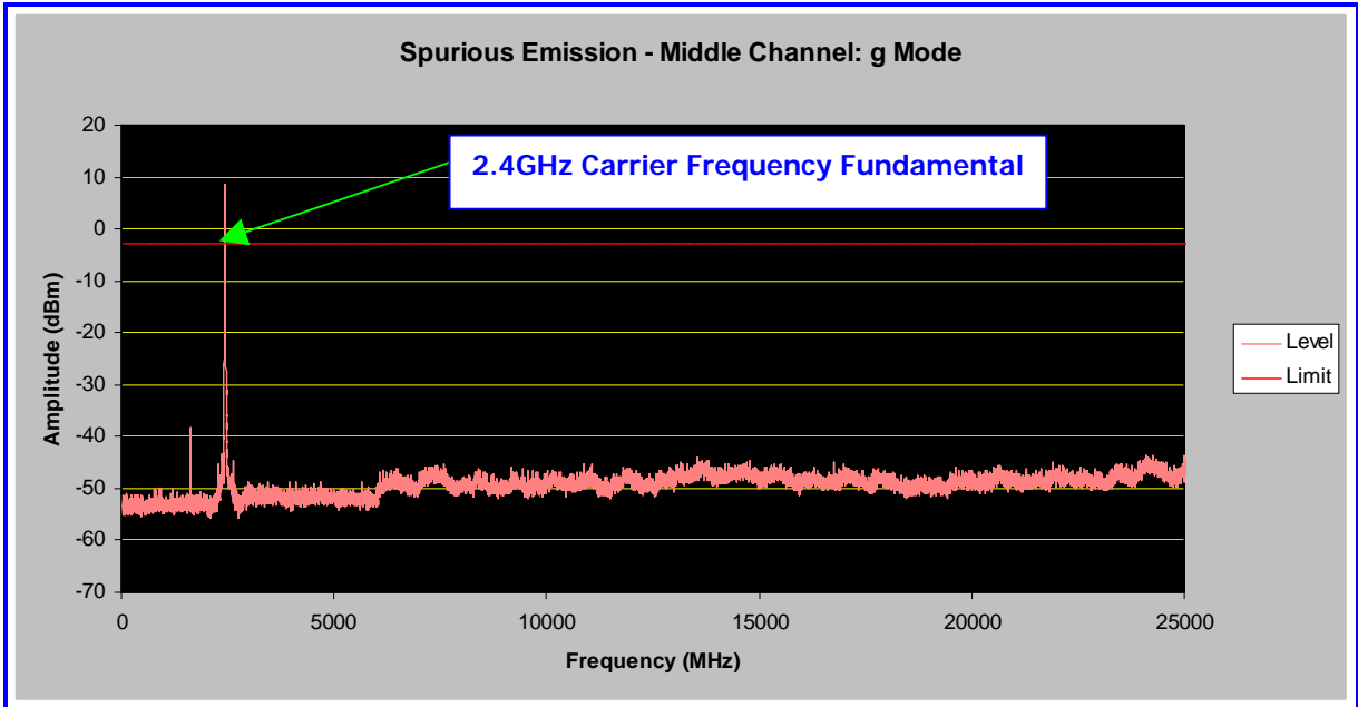
Middle Channel (802.11g)
