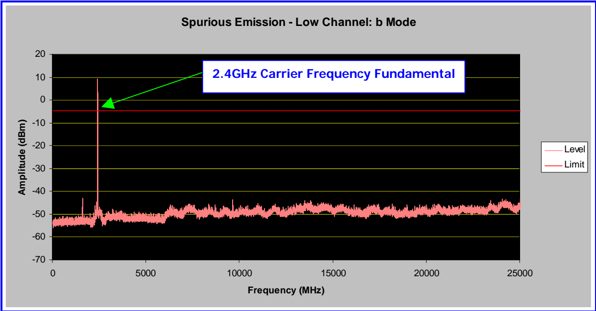
Low Channel (802.11b)
