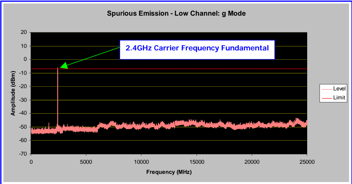
Low Channel (802.11g)
