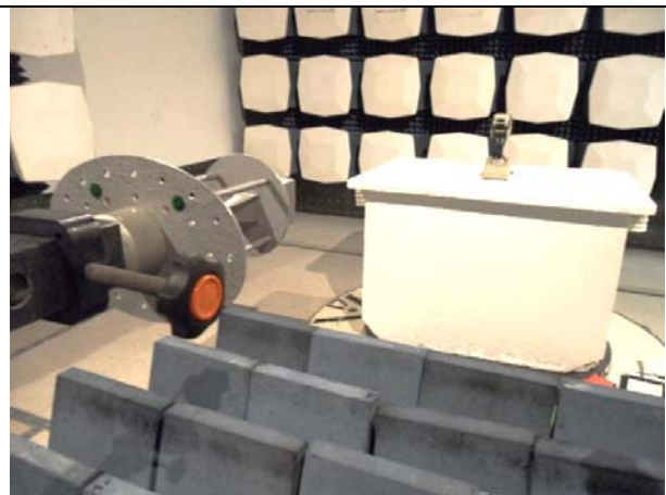
Radiated Emissions (>18GHz) – Front View
