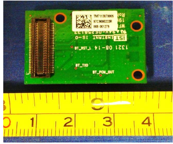
Radio Board – Bottom View
