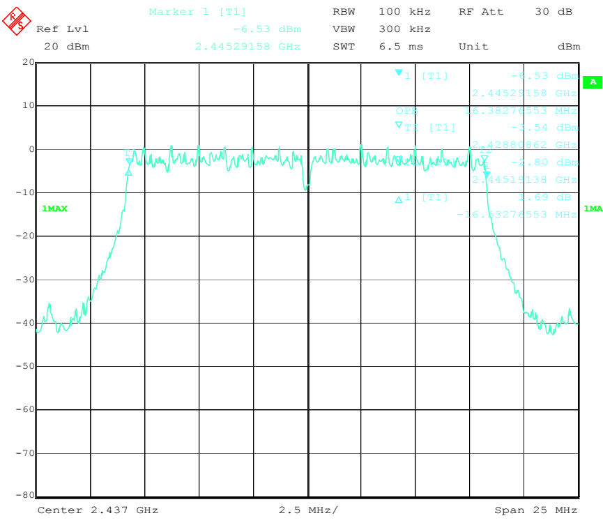
99% dB Bandwidth - 802.11g, Mid Channel
