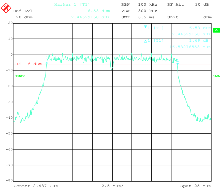
6 dB Bandwidth - 802.11g, Middle Channel
