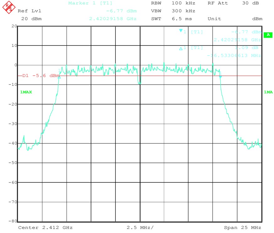
6 dB Bandwidth – 802.11g, Low Channel
