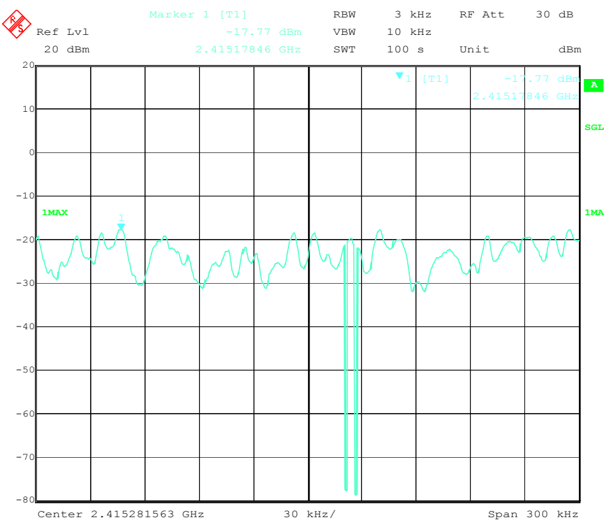
PSD Low Channel ( 802.11g)
