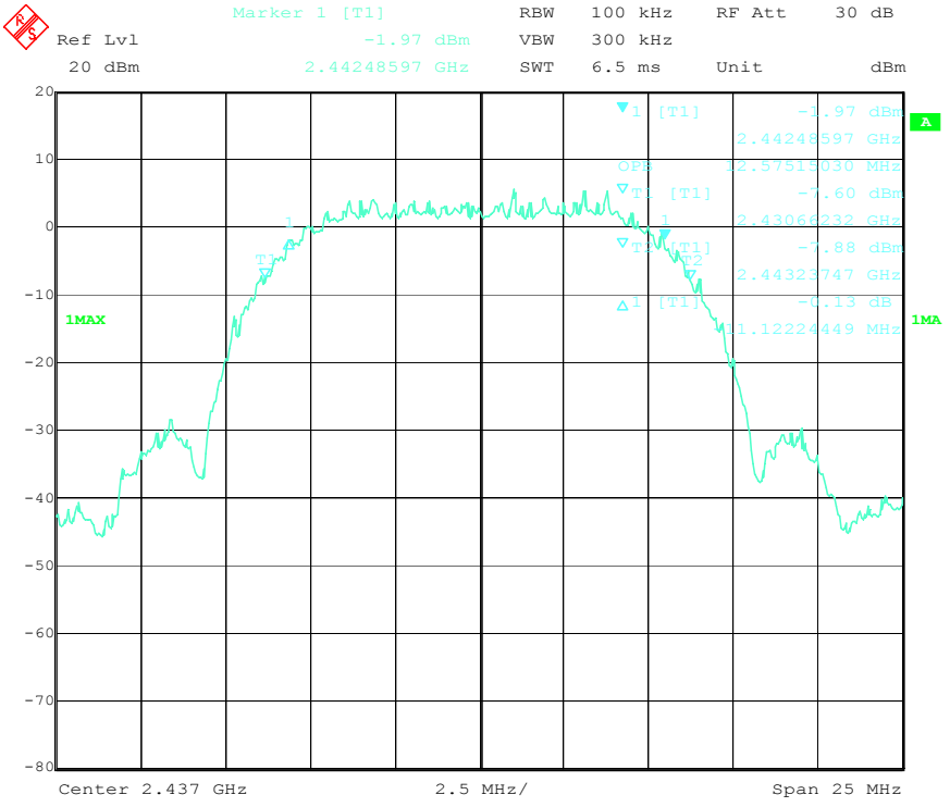
99% dB Bandwidth - 802.11b, Mid Channel
