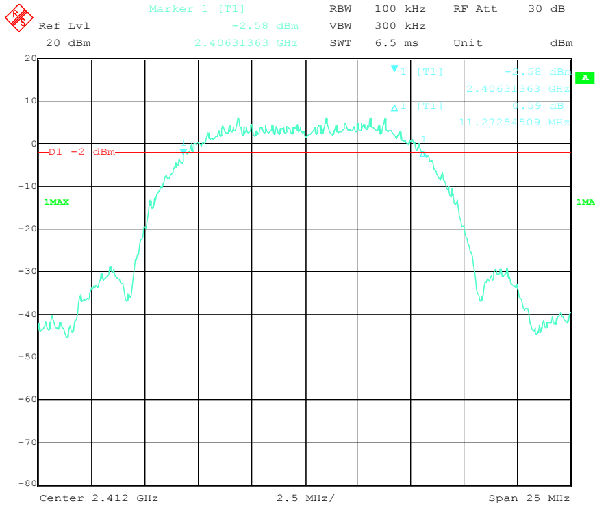
6 dB Bandwidth – 802.11b, Low Channel
