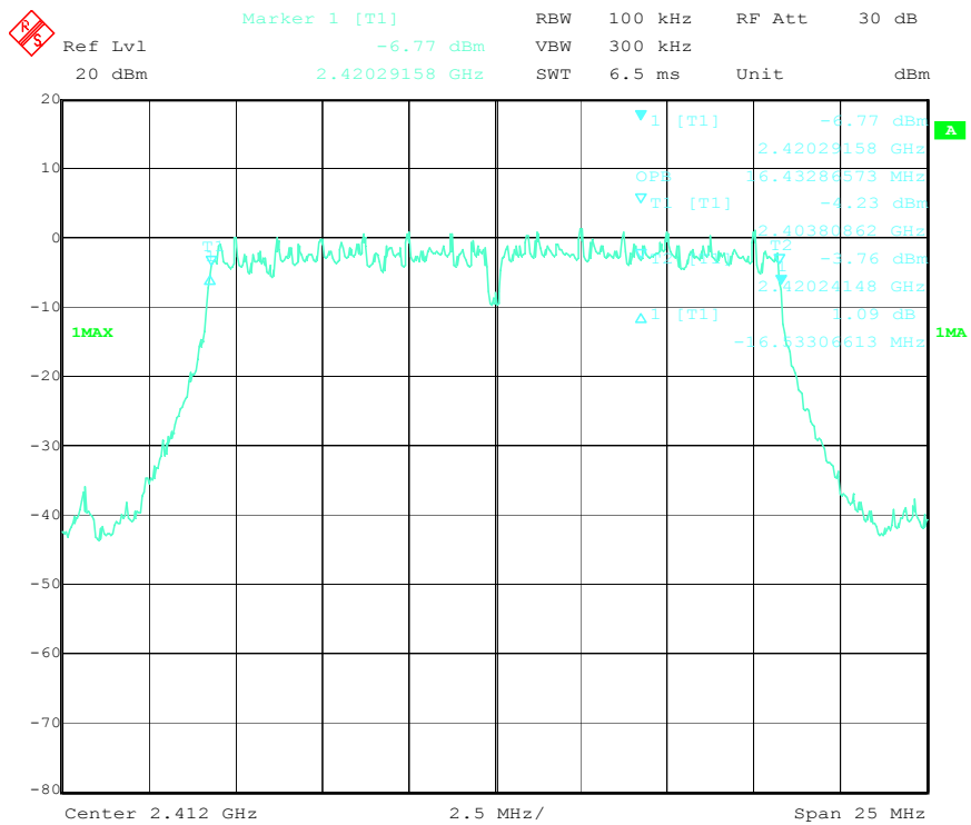
99% dB Bandwidth - 802.11g, Low Channel
