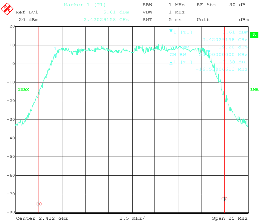
Output Power Low Channel (802.11g)
