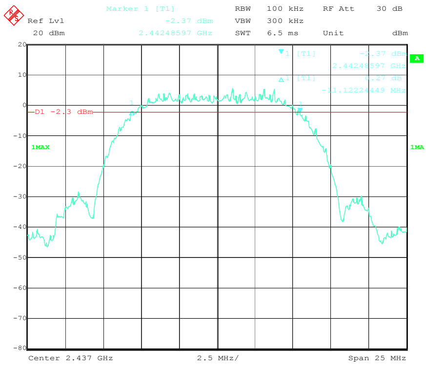
6 dB Bandwidth - 802.11b, Middle Channel
