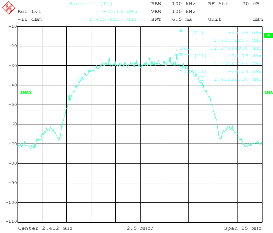
99% dB Bandwidth - 802.11b, Low Channel
