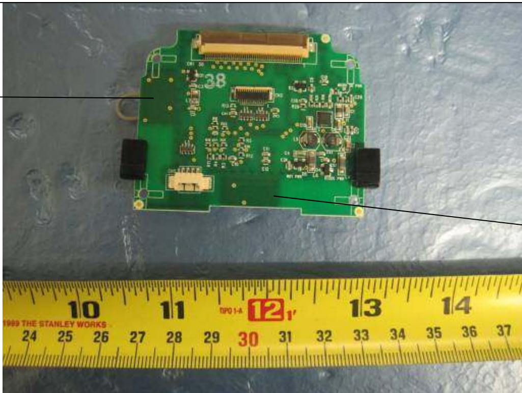
PCB A- Bottom View
