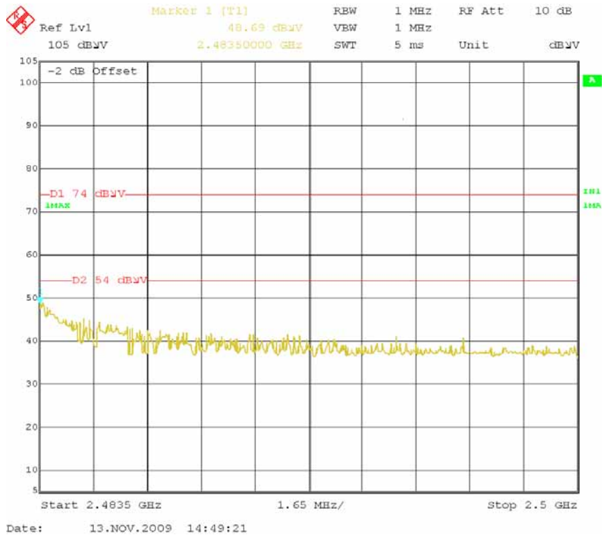
High Channel –Horizontal-Peak (802.11b)
