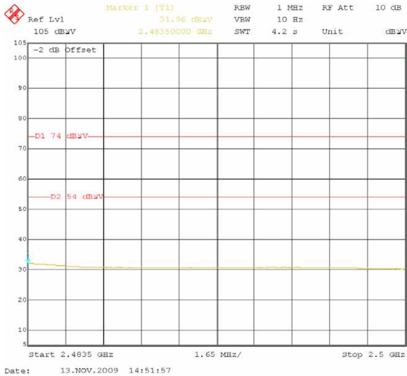
High Channel -Vertical-Average (802.11b)
