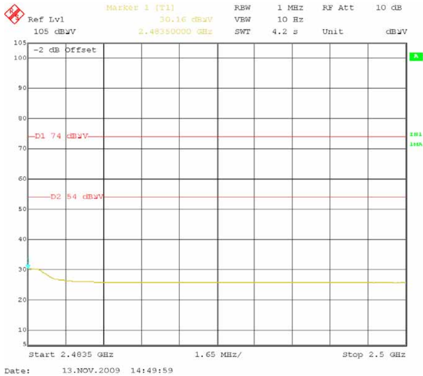
High Channel –Horizontal-Average (802.11b)
