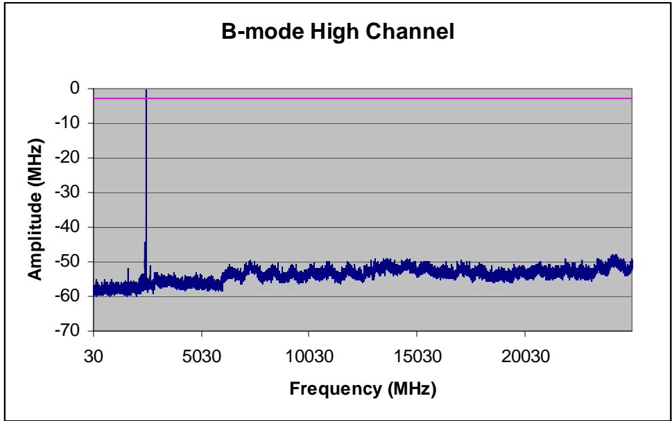
High Channel (802.11b)
