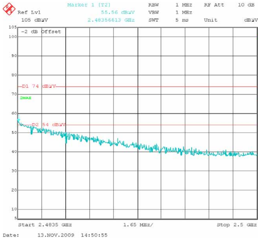
High Channel -Vertical-Peak (802.11b)
