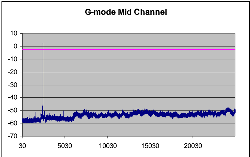
Middle Channel (802.11g)
