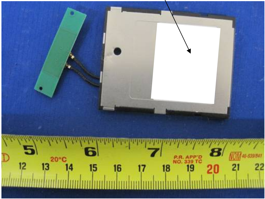
Module FCC Label Location
