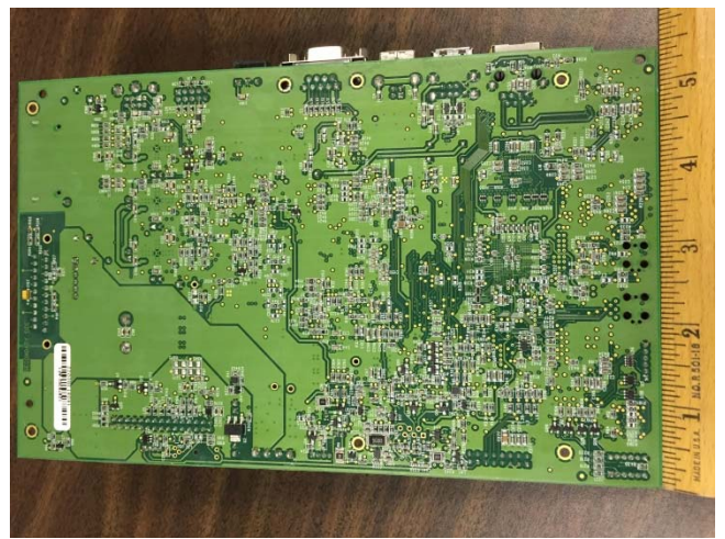
Main PCBA Board - Bottom View
