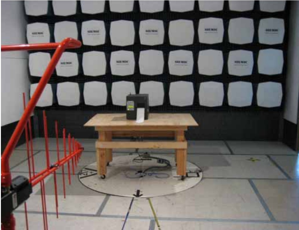
Radiated Emission Test Setup View ( 30 – 1000 MHz)
