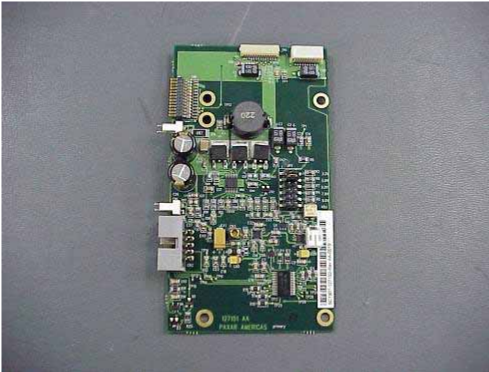
Attenuation Board Top View
