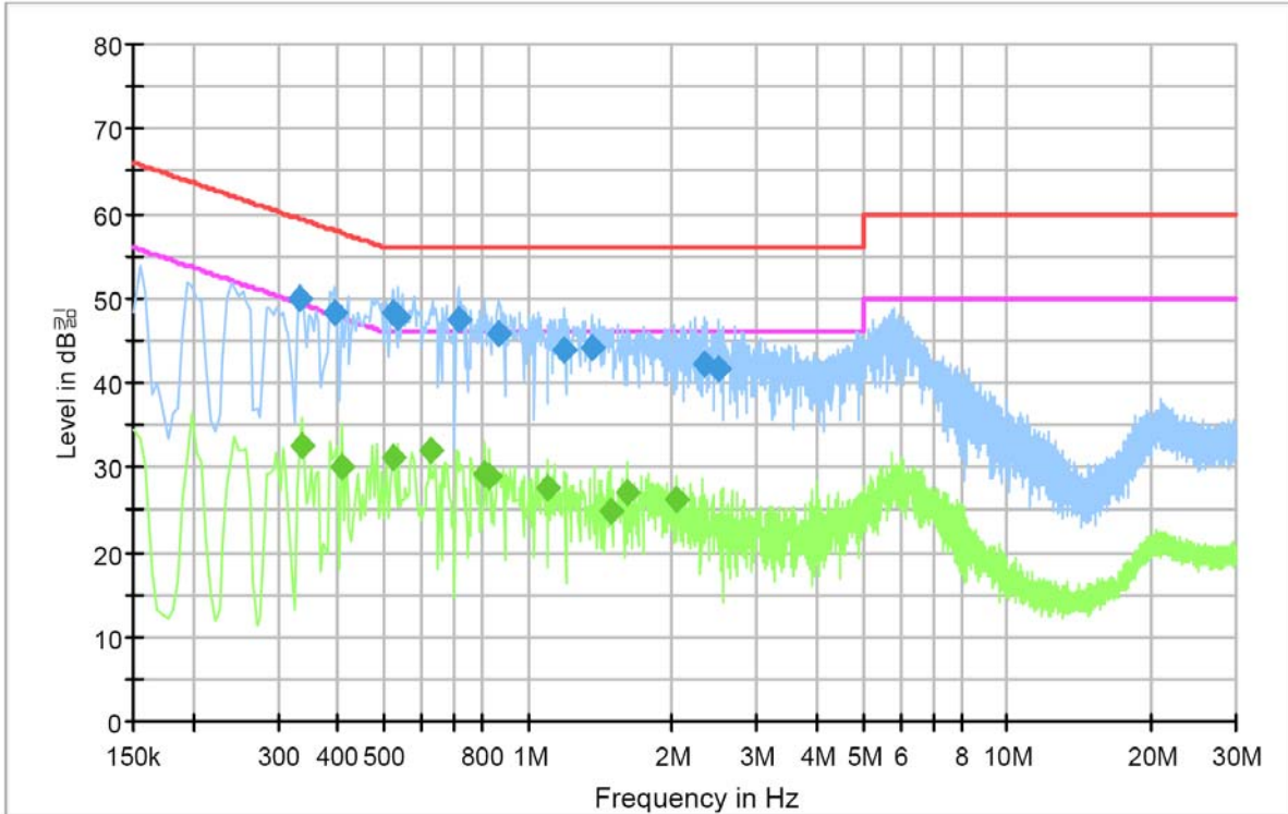
[Battery Charging Mode (Battery Charger 1): HOT]
