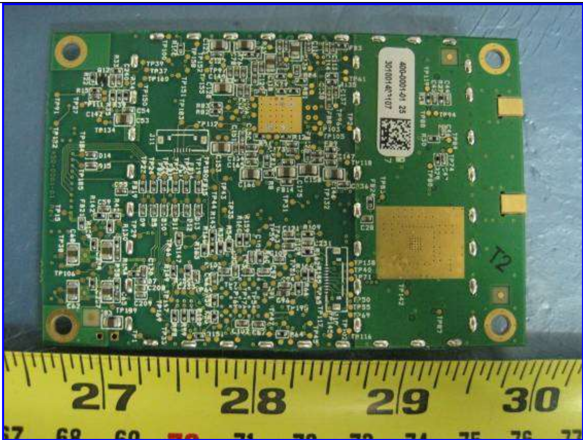
EUT (9855RFMP): RF Module PCBA Solder View
