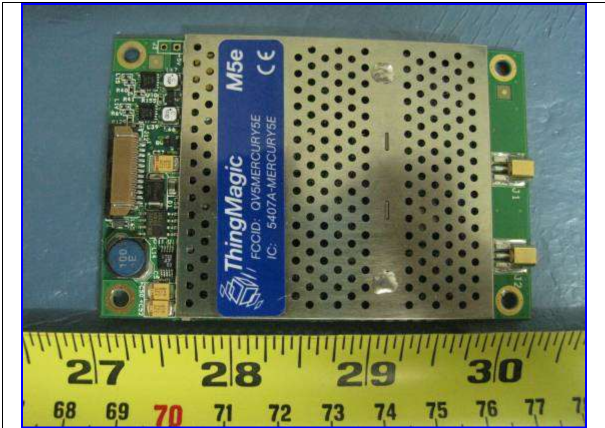
EUT :RF Module PCBA Component View (Cover On)
