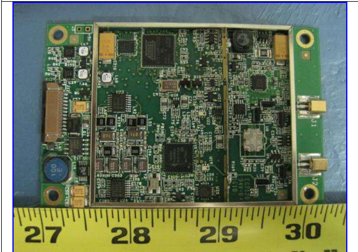
EUT : RF Module PCBA Component View (Cover Off)
