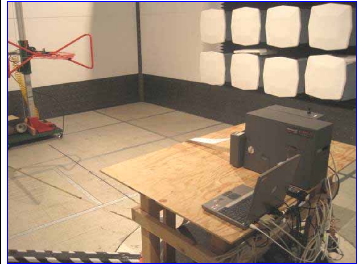
Host: 9855RFMP Radiated Emission Test Setup – Rear View
