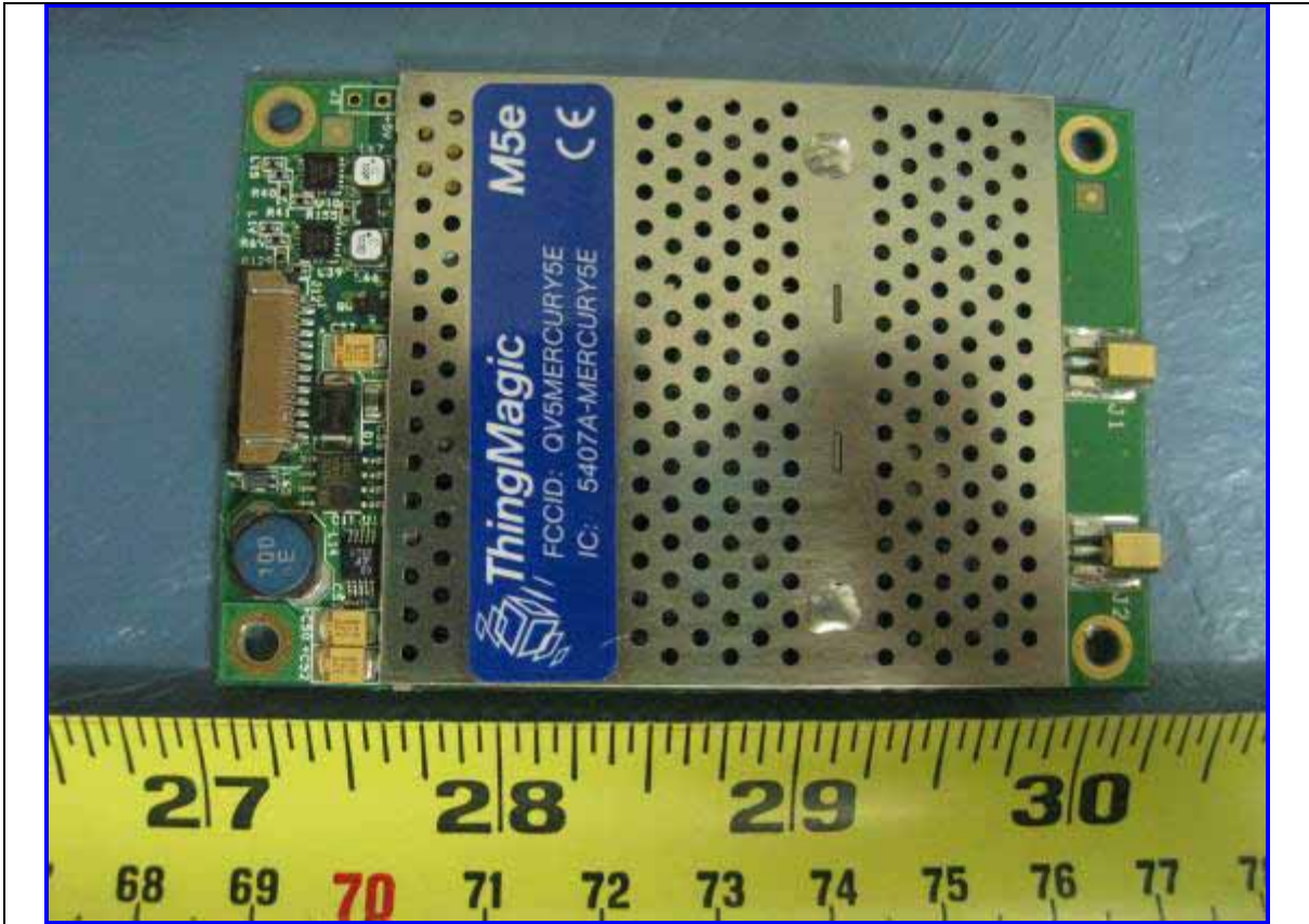
EUT (9855RFMP): RF Module PCBA Component View (Cover On)
