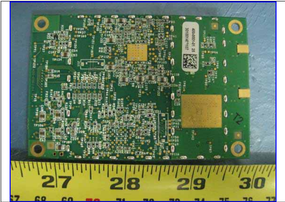
EUT (9855RFMP): RF Module PCBA Solder View
