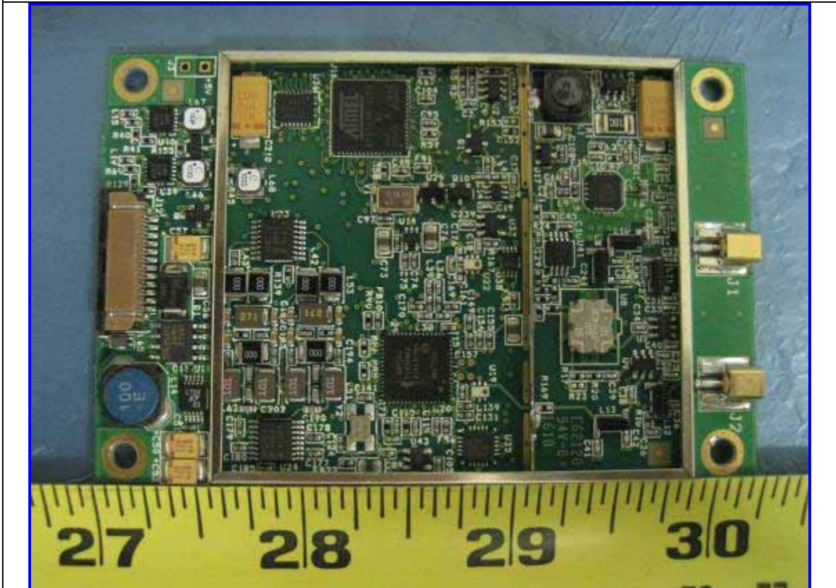
EUT (9855RFMP): RF Module PCBA Component View (Cover Off)
