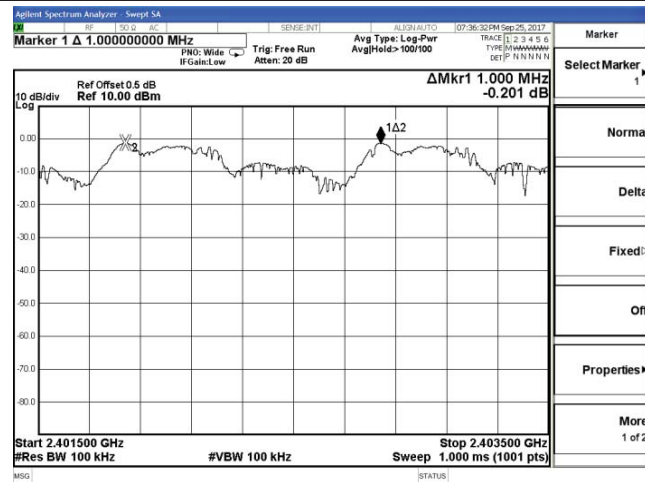
Channel 0 / 2402 MHz
