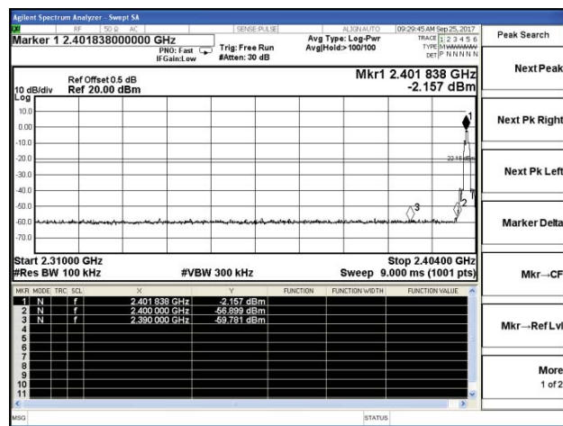
Channel 0 / 2402 MHz – Non-Hopping
