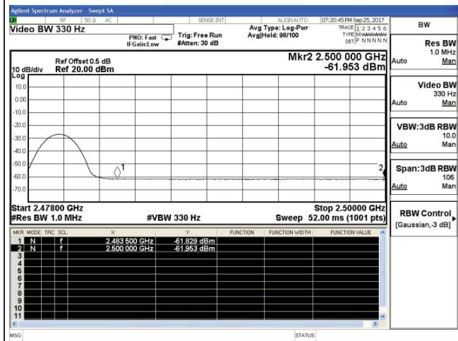
Channel 78 / 2480 MHz -Average
