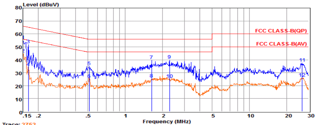
Trace: 2752 Pol:
