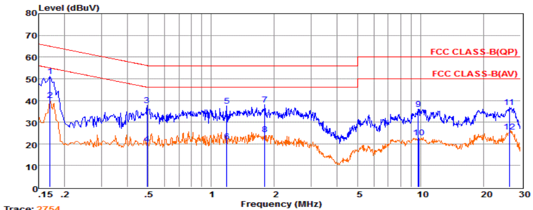
Trace: 2754 Pol:
