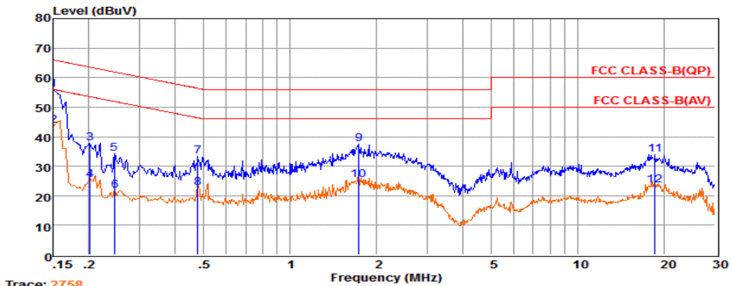
Trace: 2758 Pol:
