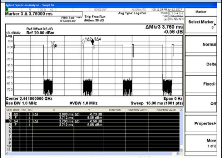
Channel 39 / 2441 MHz - 2DH5
