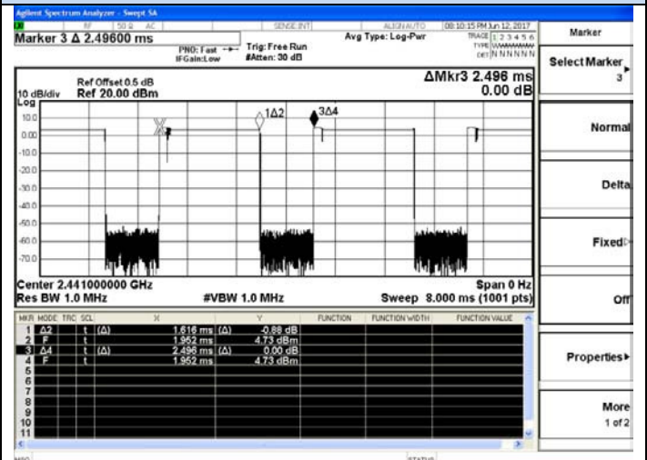
Channel 39 / 2441 MHz - 2DH3
