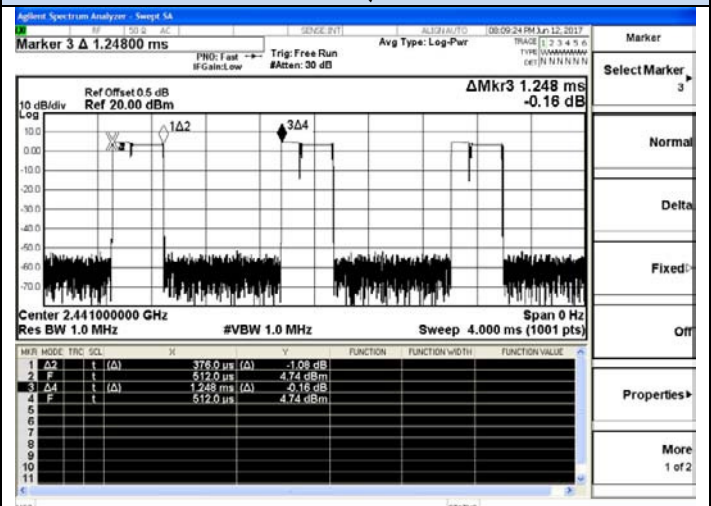
Channel 39 / 2441 MHz - 2DH1
