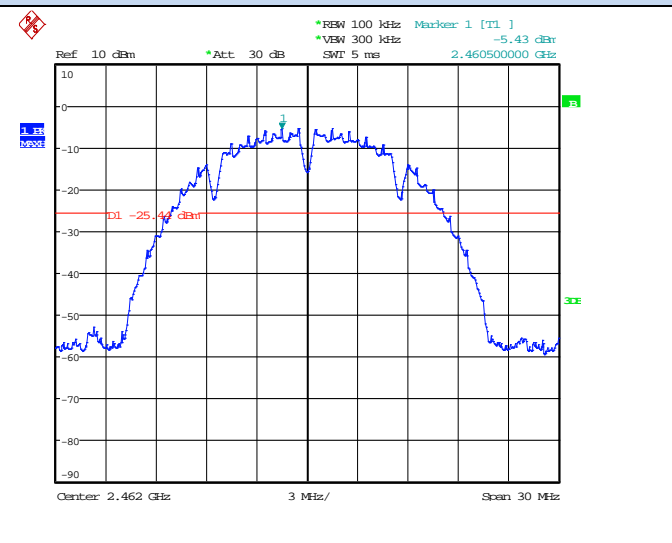
Channel 11 / 2462 MHz
