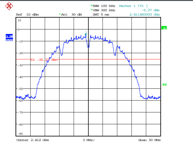
Channel 1 / 2412 MHz
