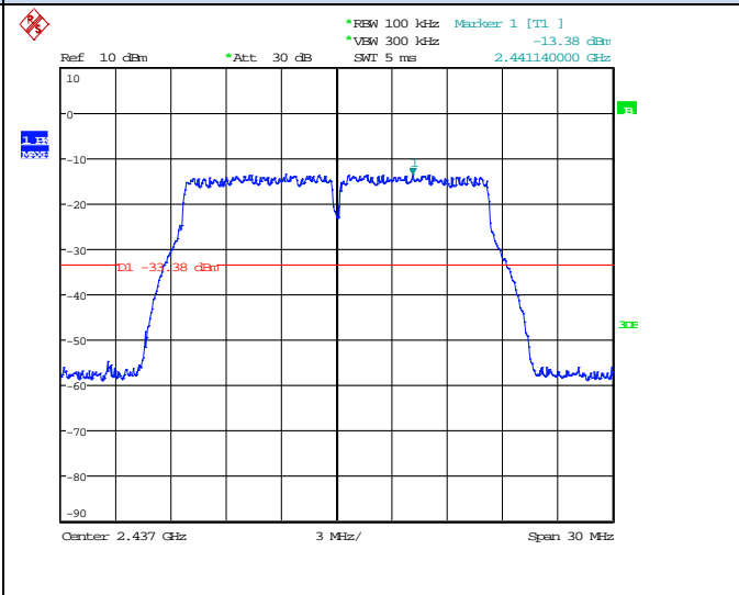
Channel 6 / 2437 MHz
