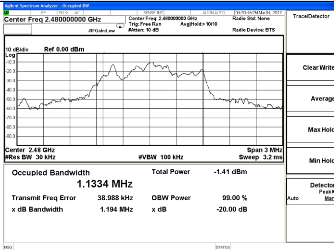
Channel 78 / 2480 MHz
