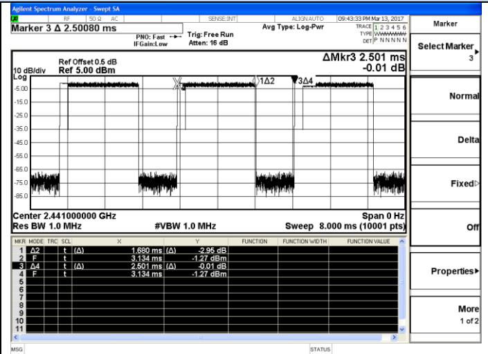
2 Channel 39 / 2441 MHz - 3DH3
