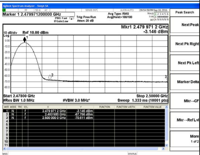
BT LE-High channel(Average)
