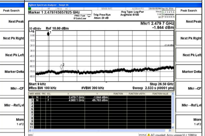
BT LE-High channel
