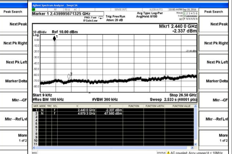
BT LE-Middle channel
