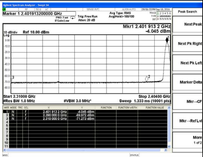
BT LE-Low channel(Average)
