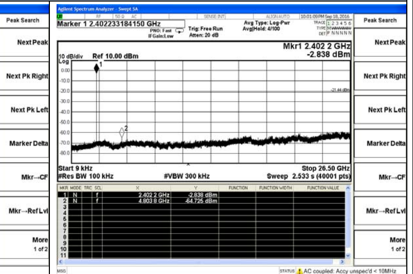
BT LE-Low channel
