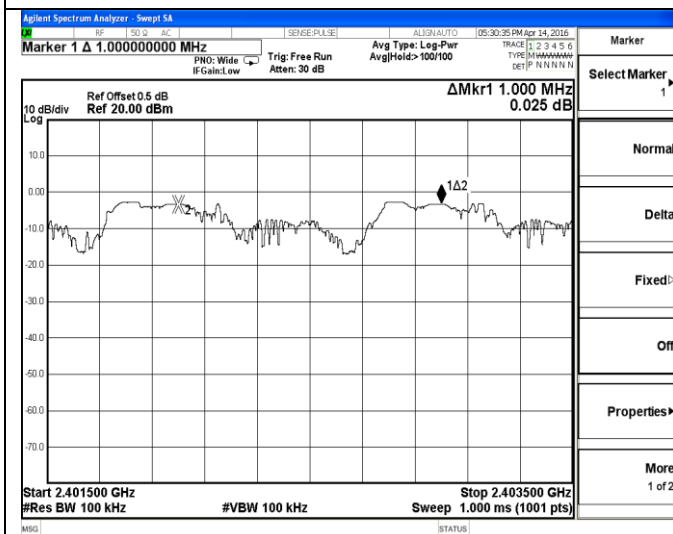
Test plot of Frequency Separation-3Mbps
