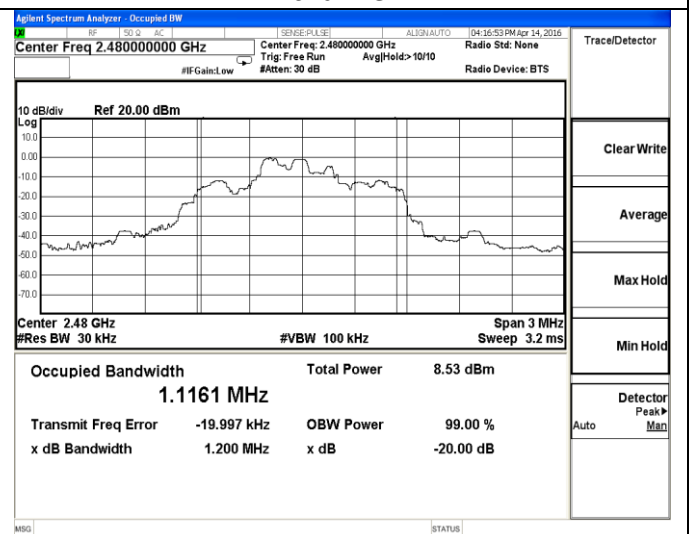
Test plot of 20dB Bandwidth-3Mbps-High channel
