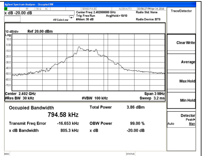
Test plot of 20dB Bandwidth-1Mbps-Low channel
