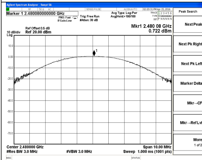
3DH1-High channel
