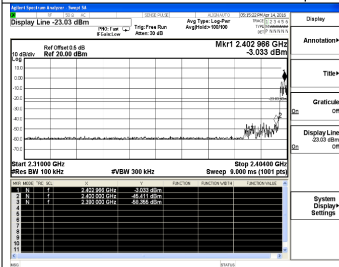
Hopping On-8-DPSK-Low channel
