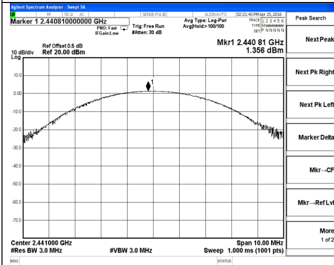
3DH1-Middle channel
