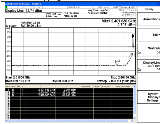
Hopping Off-GFSK-Low channel
