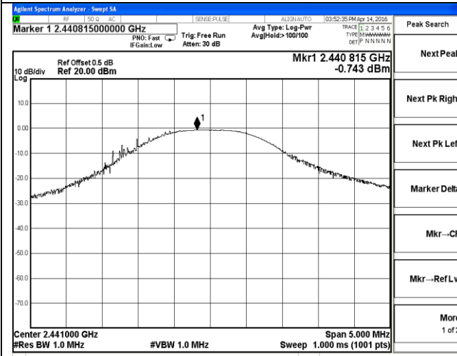
DH1-Middle channel
