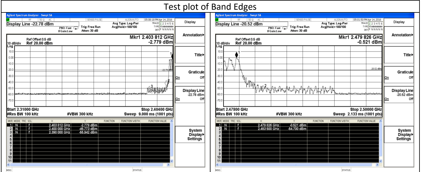
Hopping On-GFSK-Low channel
