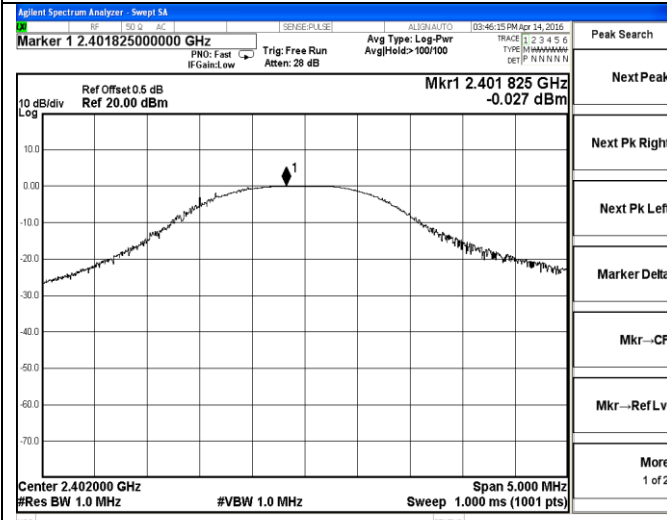
DH1-Low channel
