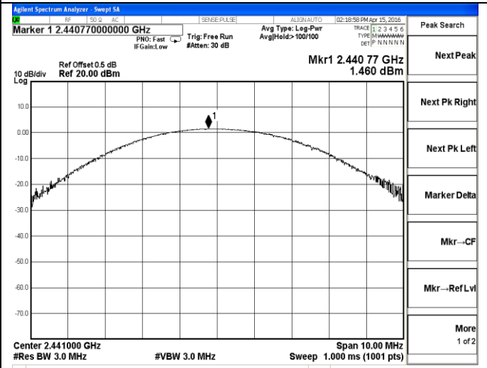
2DH1-Middle channel
