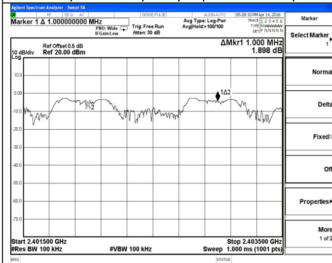
Test plot of Frequency Separation-2Mbps
