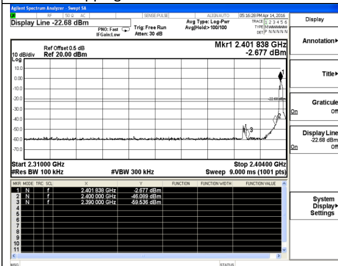
Hopping Off-8-DPSK-Low channel
