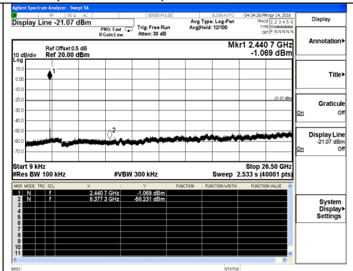
3DH1-Middle channel
