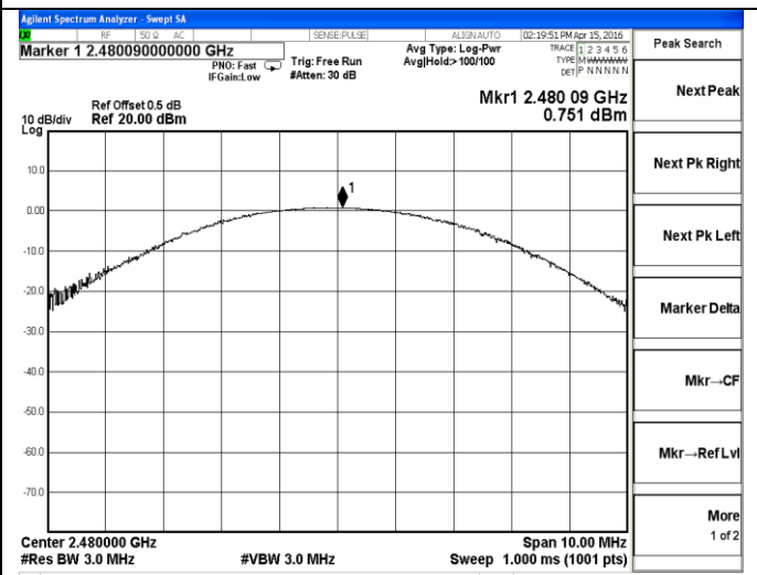
2DH1-High channel
