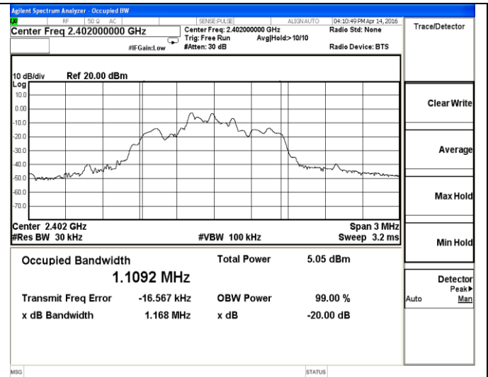
Test plot of 20dB Bandwidth-3Mbps-Low channel
