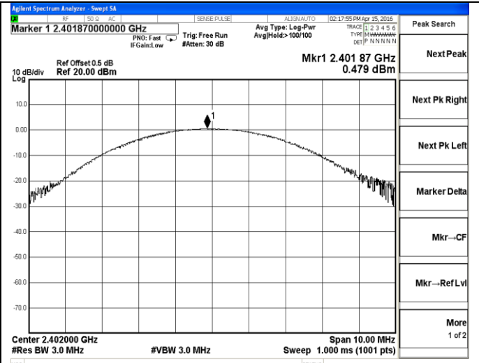
2DH1-Low channel
