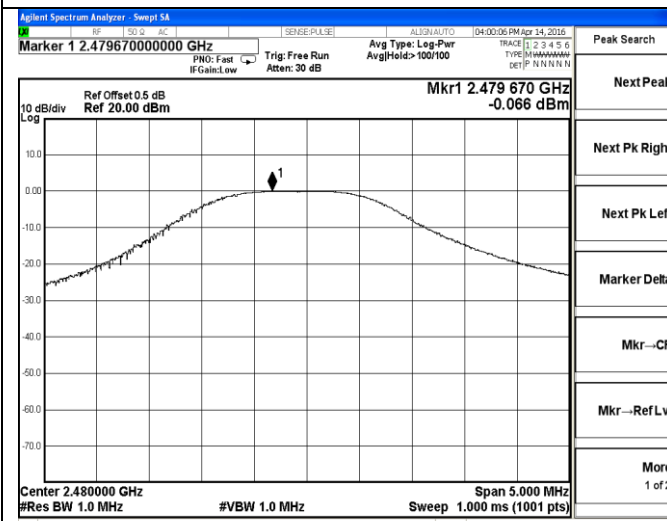
DH1-High channel
