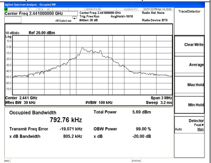
Test plot of 20dB Bandwidth-1Mbps-Middle channel
