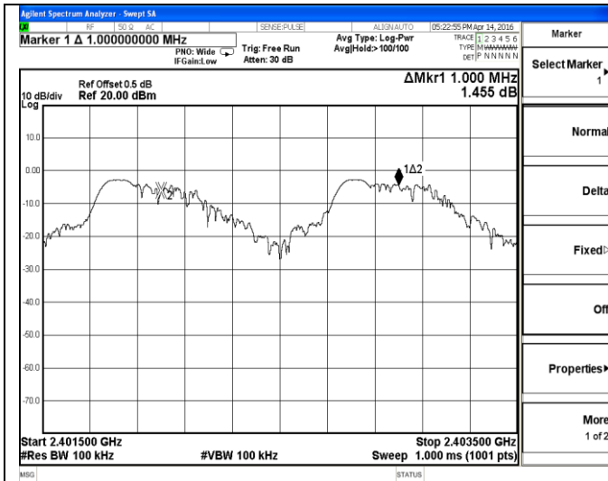
Test plot of Frequency Separation-1Mbps
