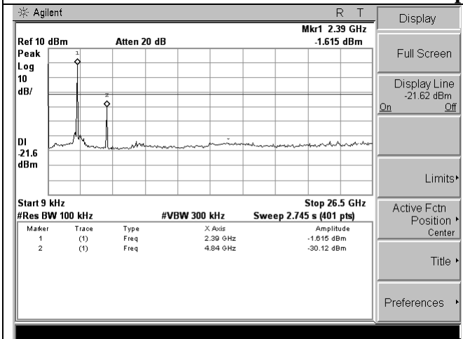
Test frequency: 2402MHz(GFSK)
