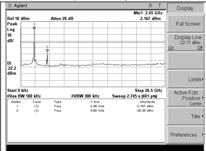
Test frequency: 2441MHz(GFSK)
