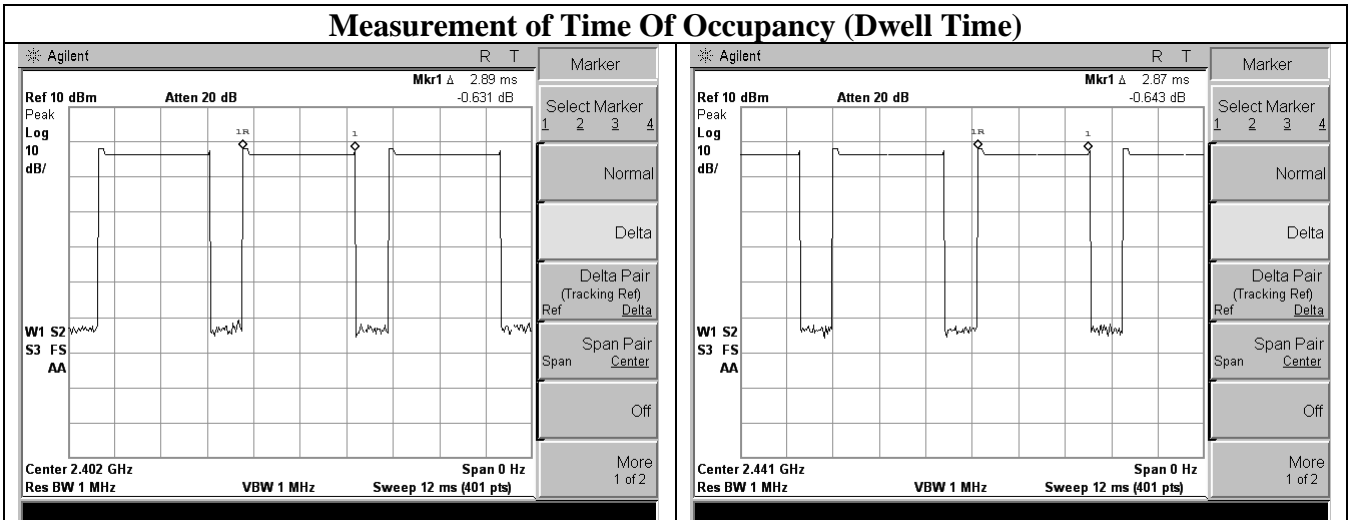
Test frequency: 2402MHz(GFSK)
