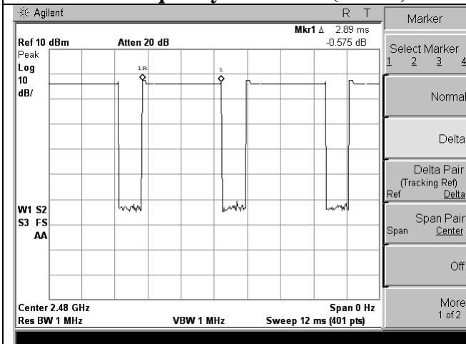
Test frequency: 2480MHz(GFSK)
