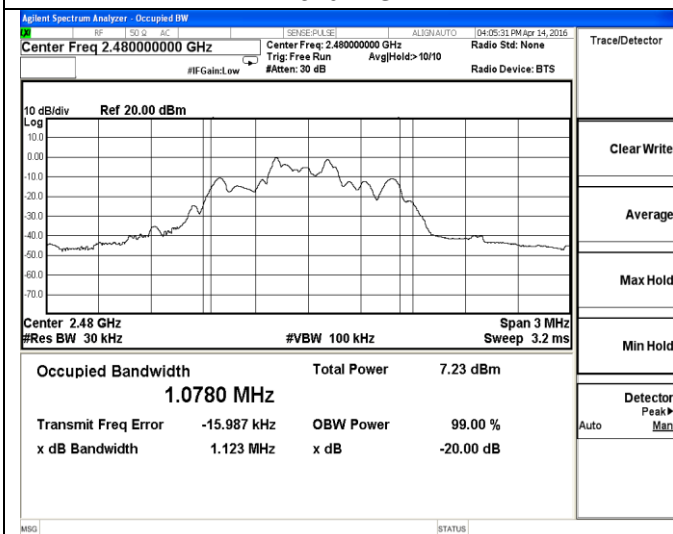
Test plot of 20dB Bandwidth-2Mbps-High channel
