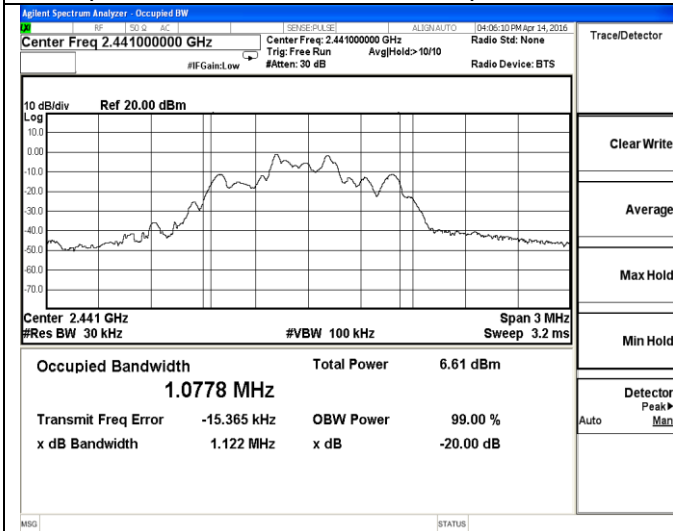
Test plot of 20dB Bandwidth-2Mbps-Middle channel
