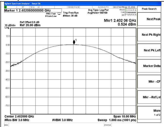
2DH1-Low channel
