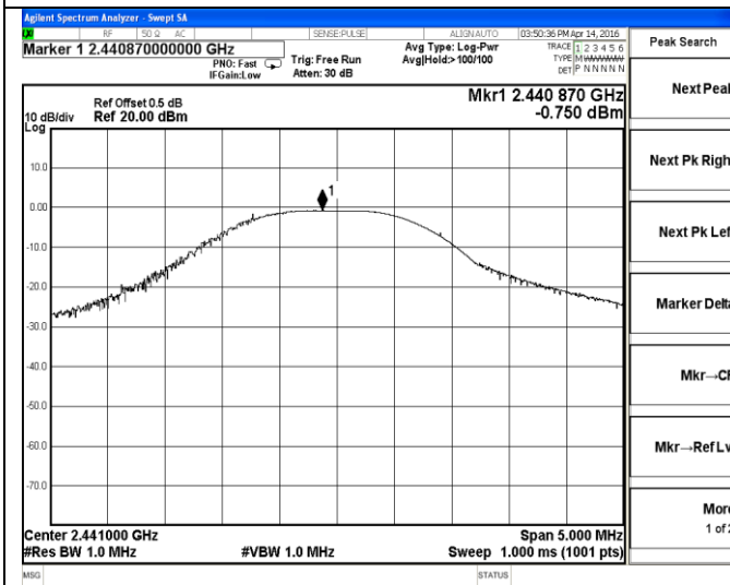
DH1-Middle channel
