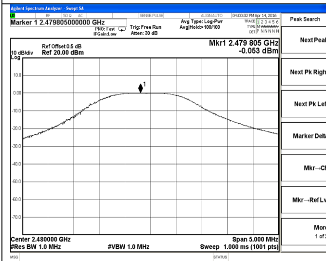
DH1-High channel
