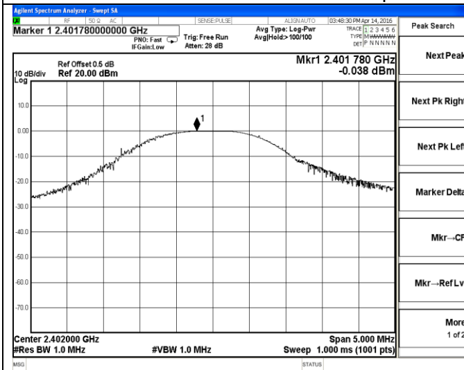
DH1-Low channel
