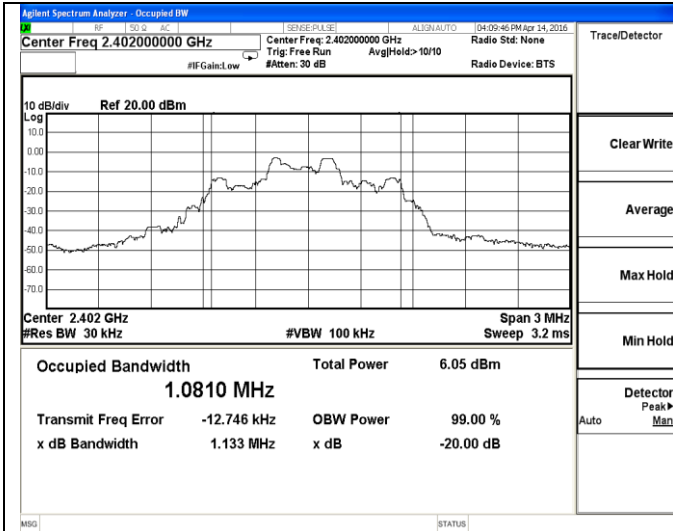
Test plot of 20dB Bandwidth-2Mbps-Low channel
