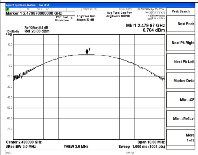
2DH1-High channel
