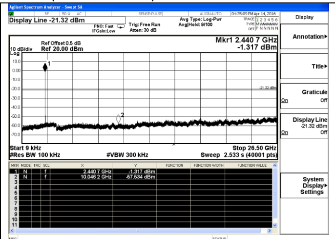
3DH1-Middle channel
