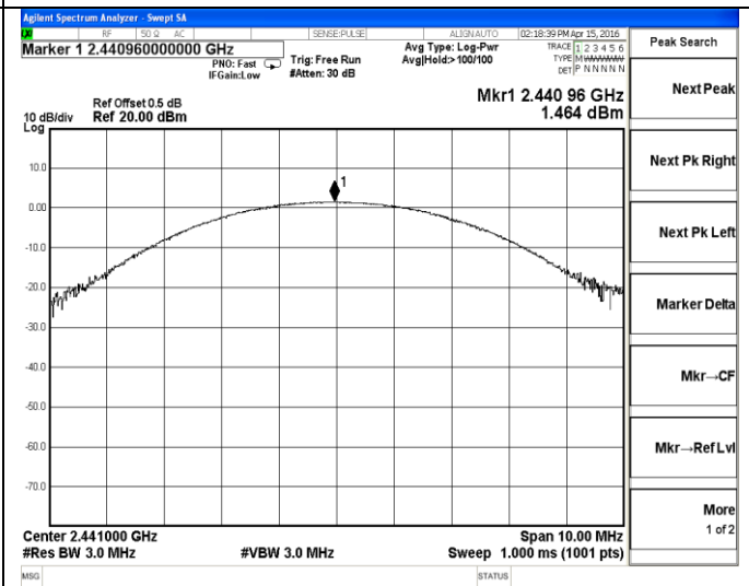
2DH1-Middle channel
