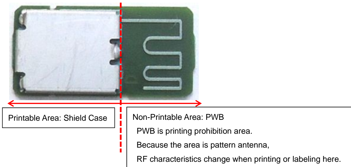
BTS04 module External View
