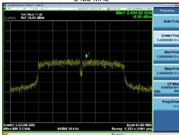
2422 MHz
