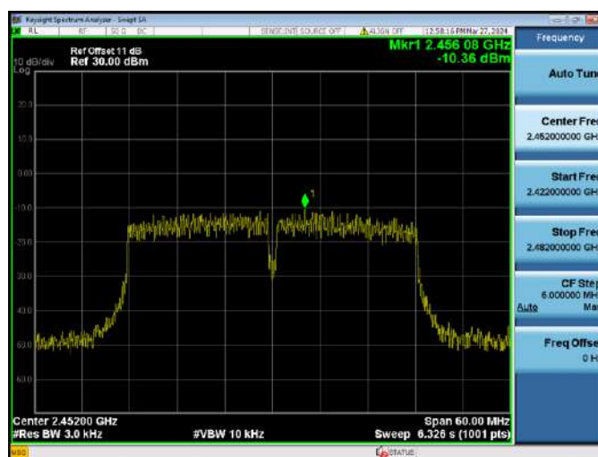
2452 MHz
