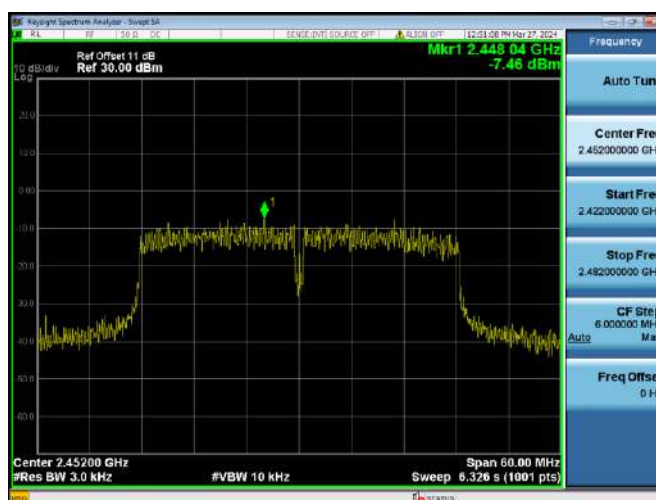
2452 MHz
