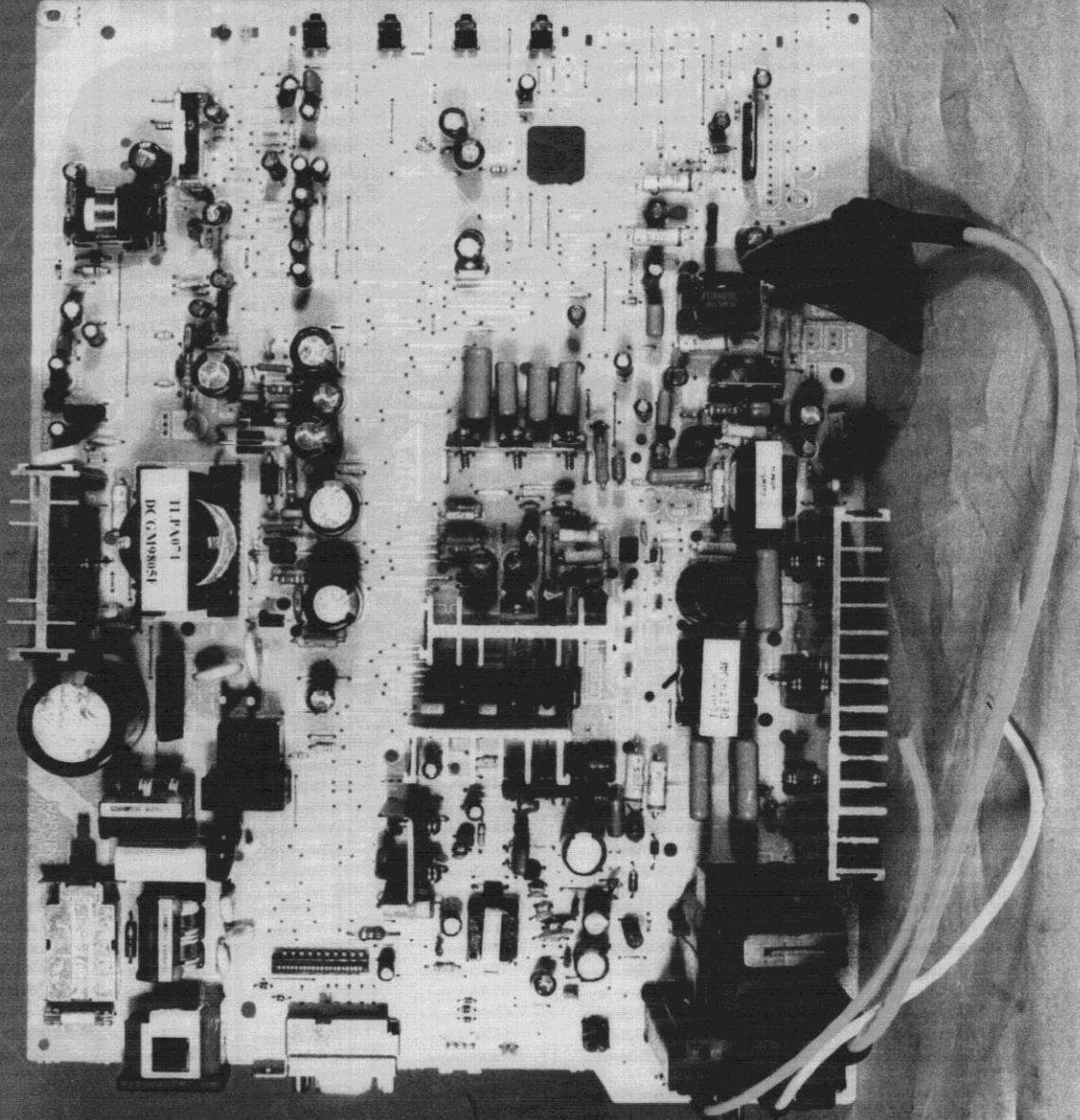
Photo. 4. Main & Power Supply PWB of Model VCCTS21406-2*
