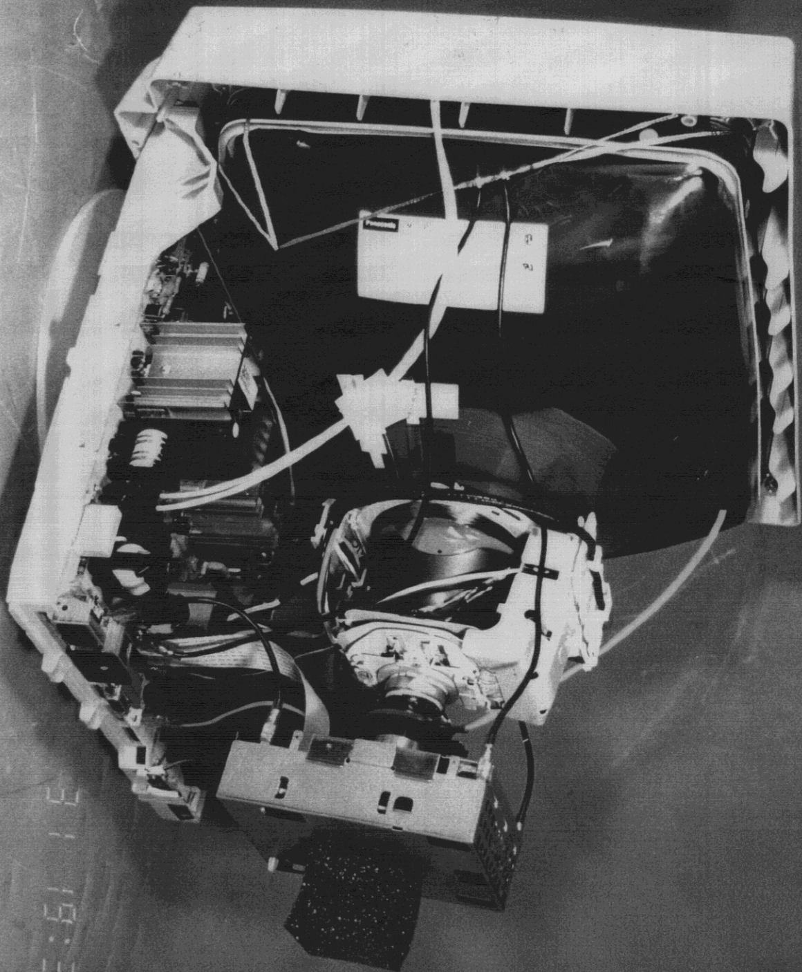
Fig.3. Inside view (without shield case) of VCRMS01A33 **
