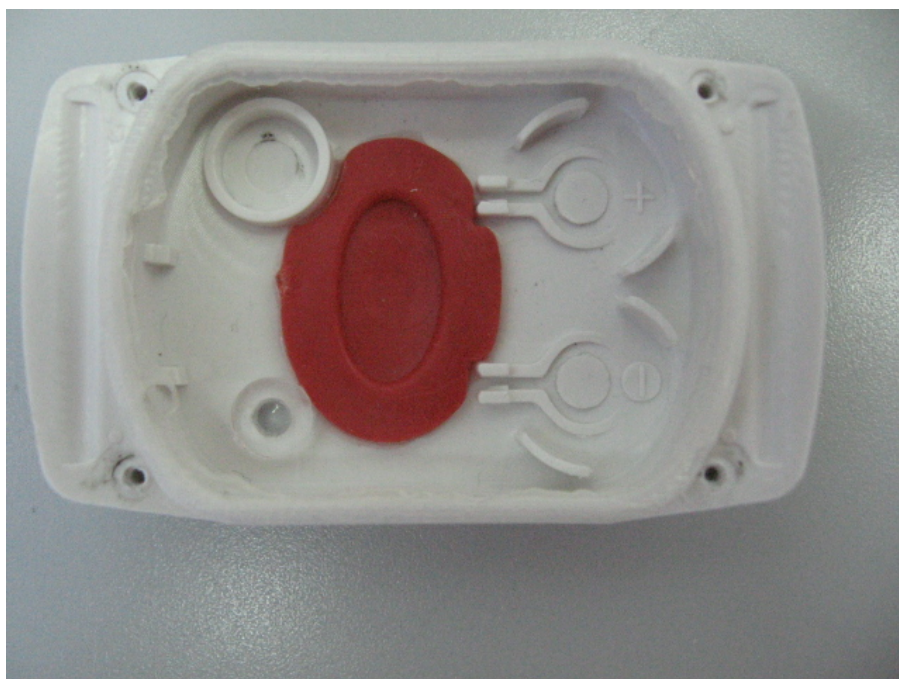
Figure 2 Top Cover Internal View
