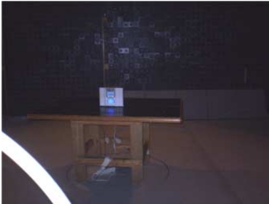
Photograph No.1 Setup for spurious emission field strength measurements in anechoic chamber below 30 MHz
