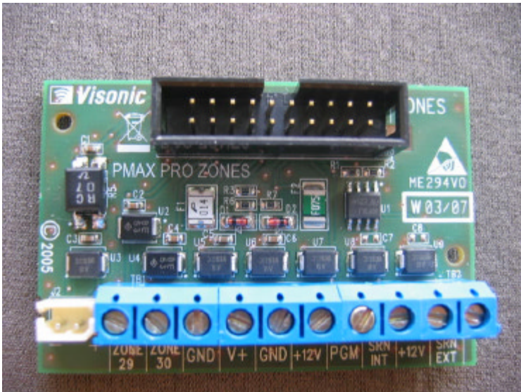
Photograph No.22 Zones PCB frontview
