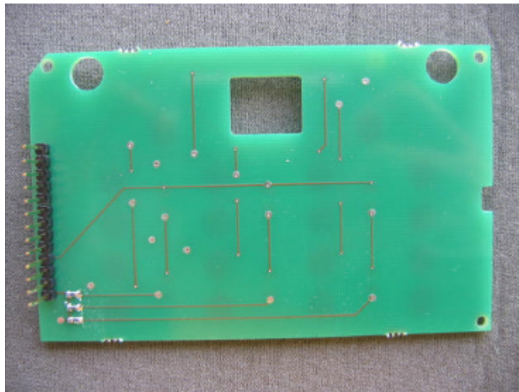
Photograph No.21 Display PCB second sideview
