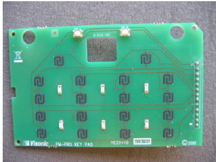
Photograph No.20 Display PCB front view
