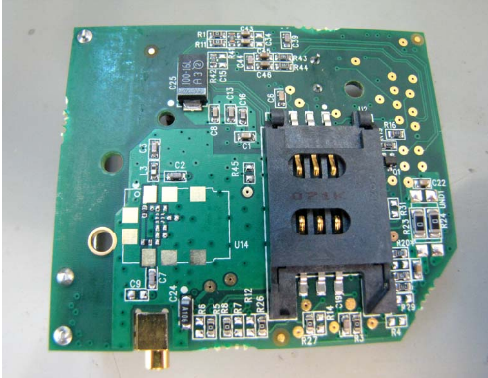
Photograph No.8 GSM modem main PCB front view
