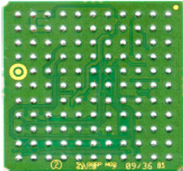
Photograph No.11 GE864-Quad V2 module PCB second side view
