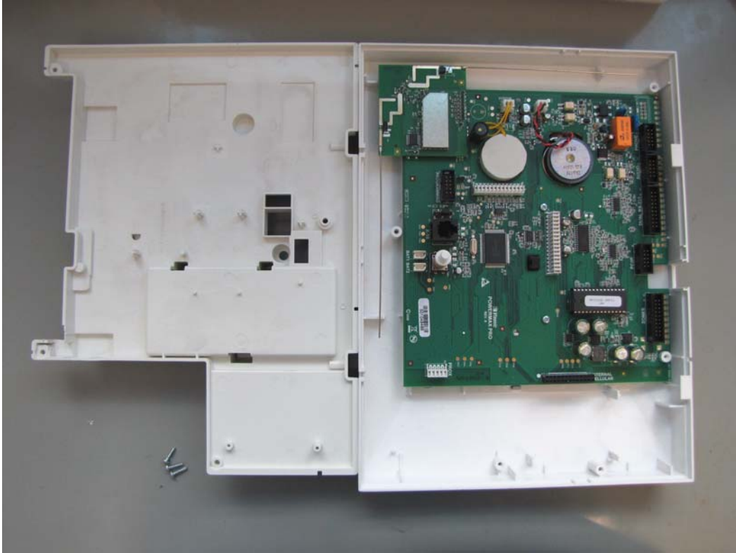
Photograph No.4 PowerMax Pro main part with cover removed view
