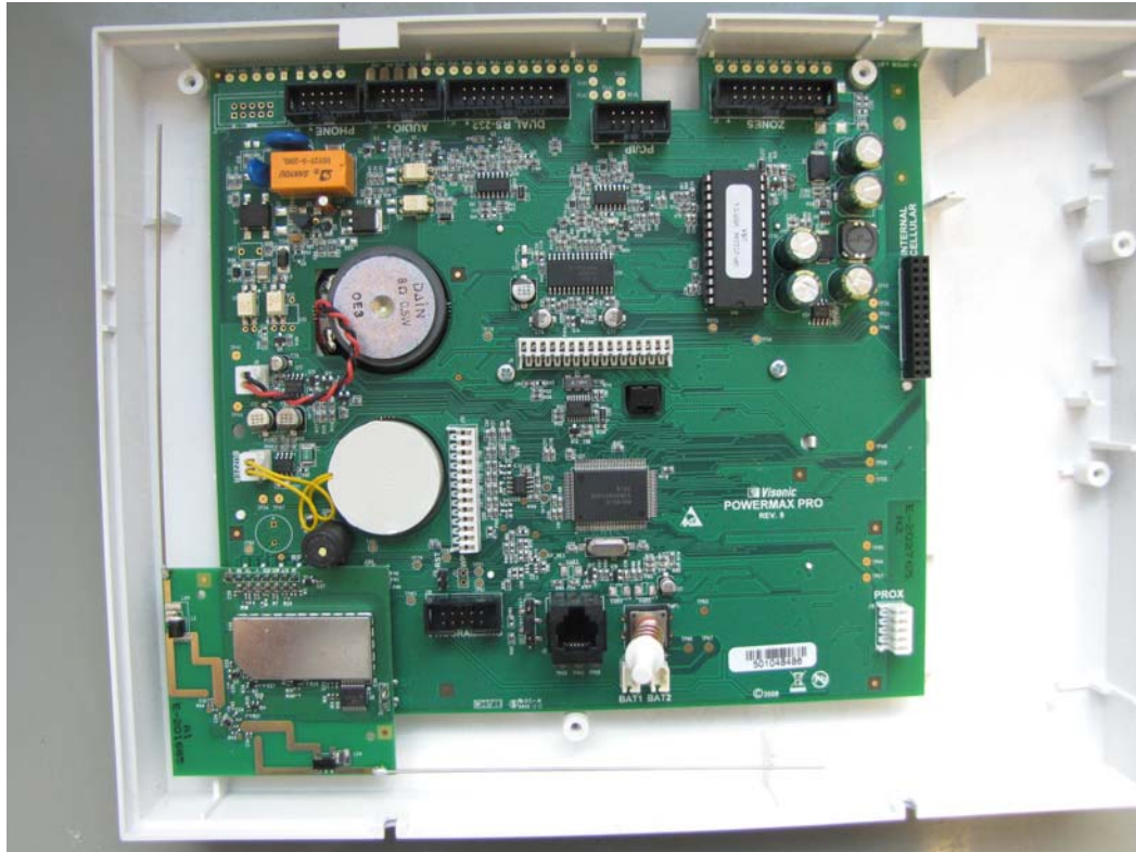
Photograph No.5 PowerMax Pro main PCB view
