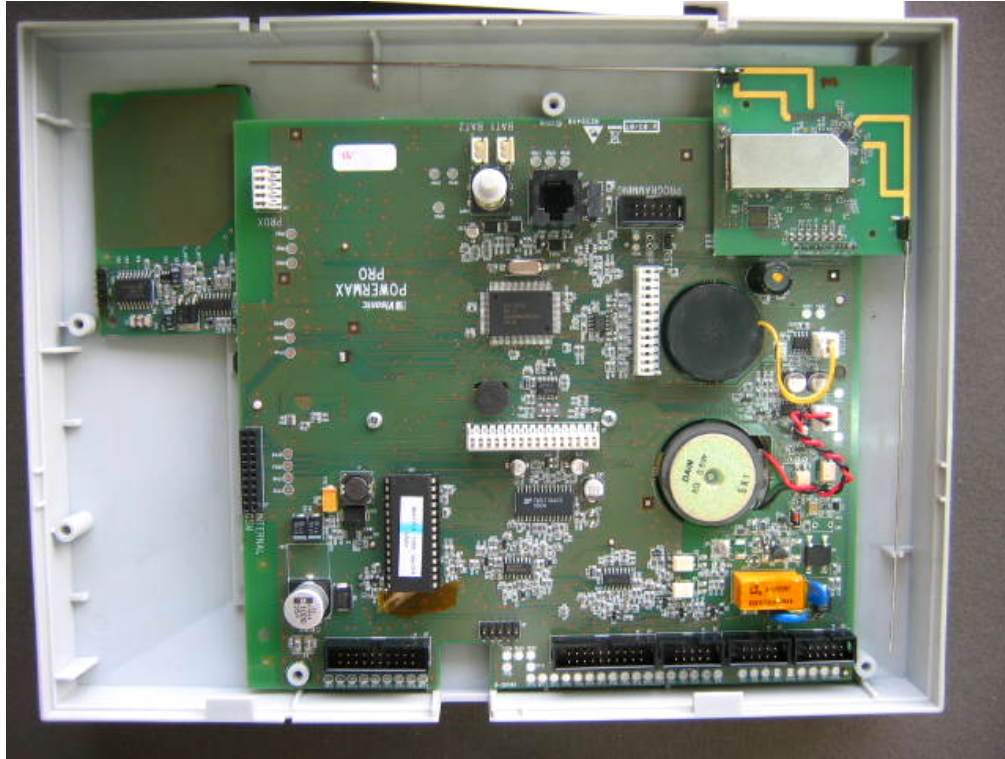
Photograph No.5 PowerMax Pro main PCB view
