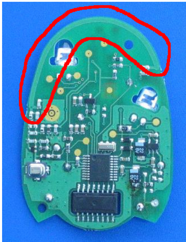
Photograph 7.4.1 Antenna assembly
