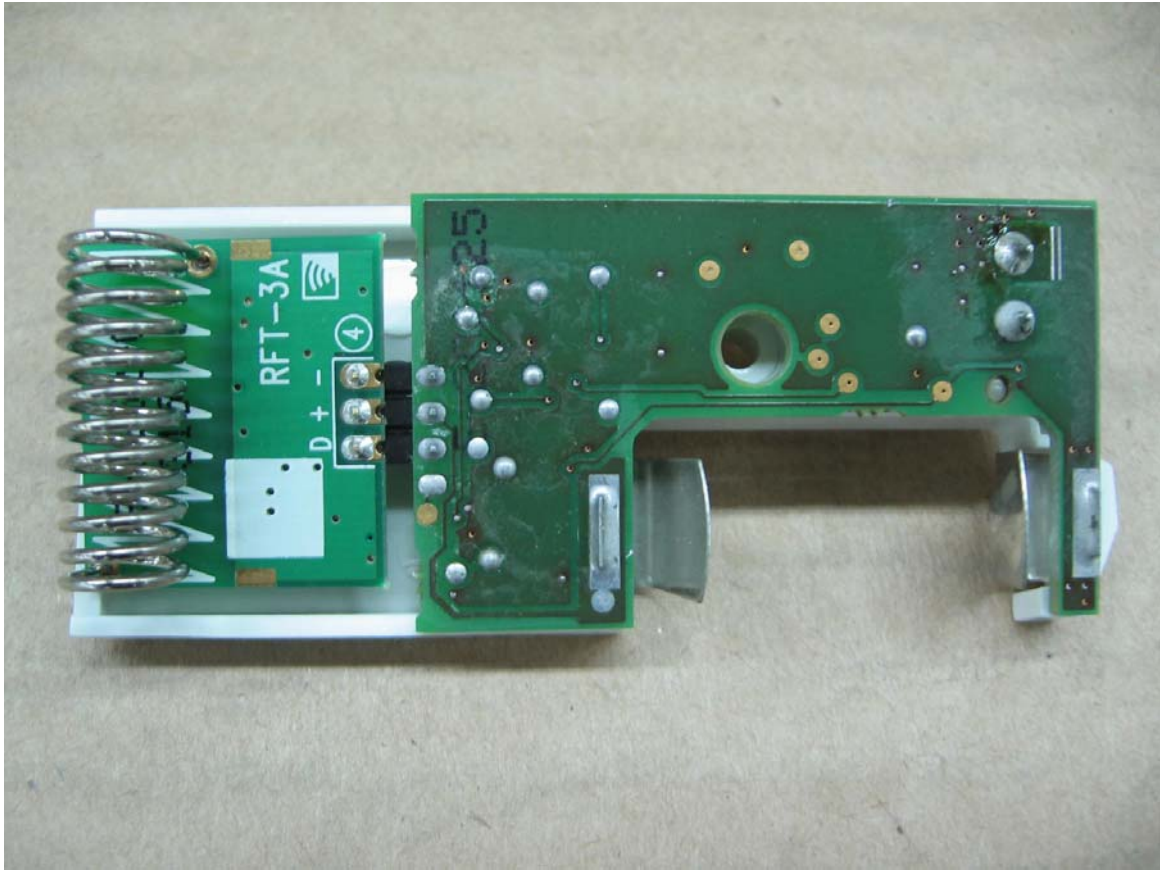
Figure 1: Inside of Unit bottom side of PCB
