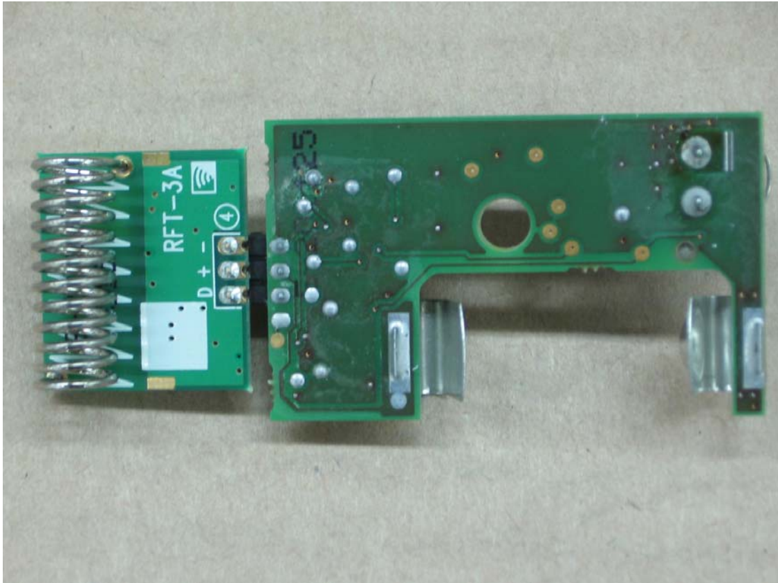
Figure 3: Bottom side of PCB
