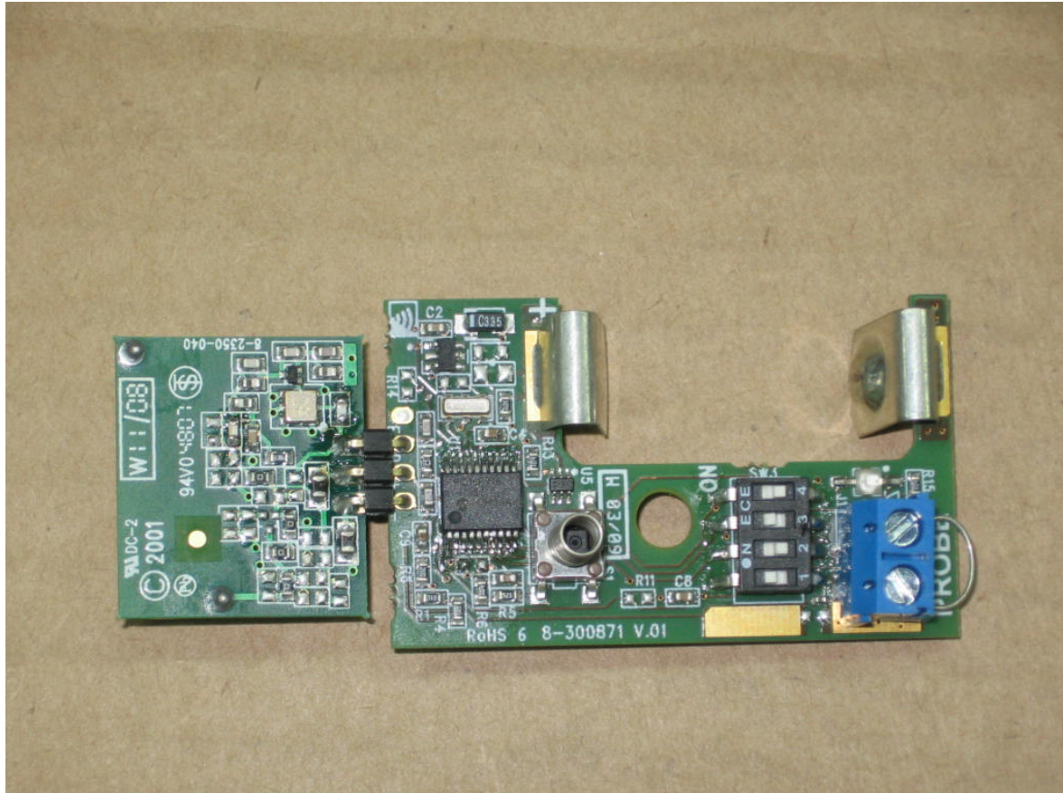
Figure 2: top side of PCB
