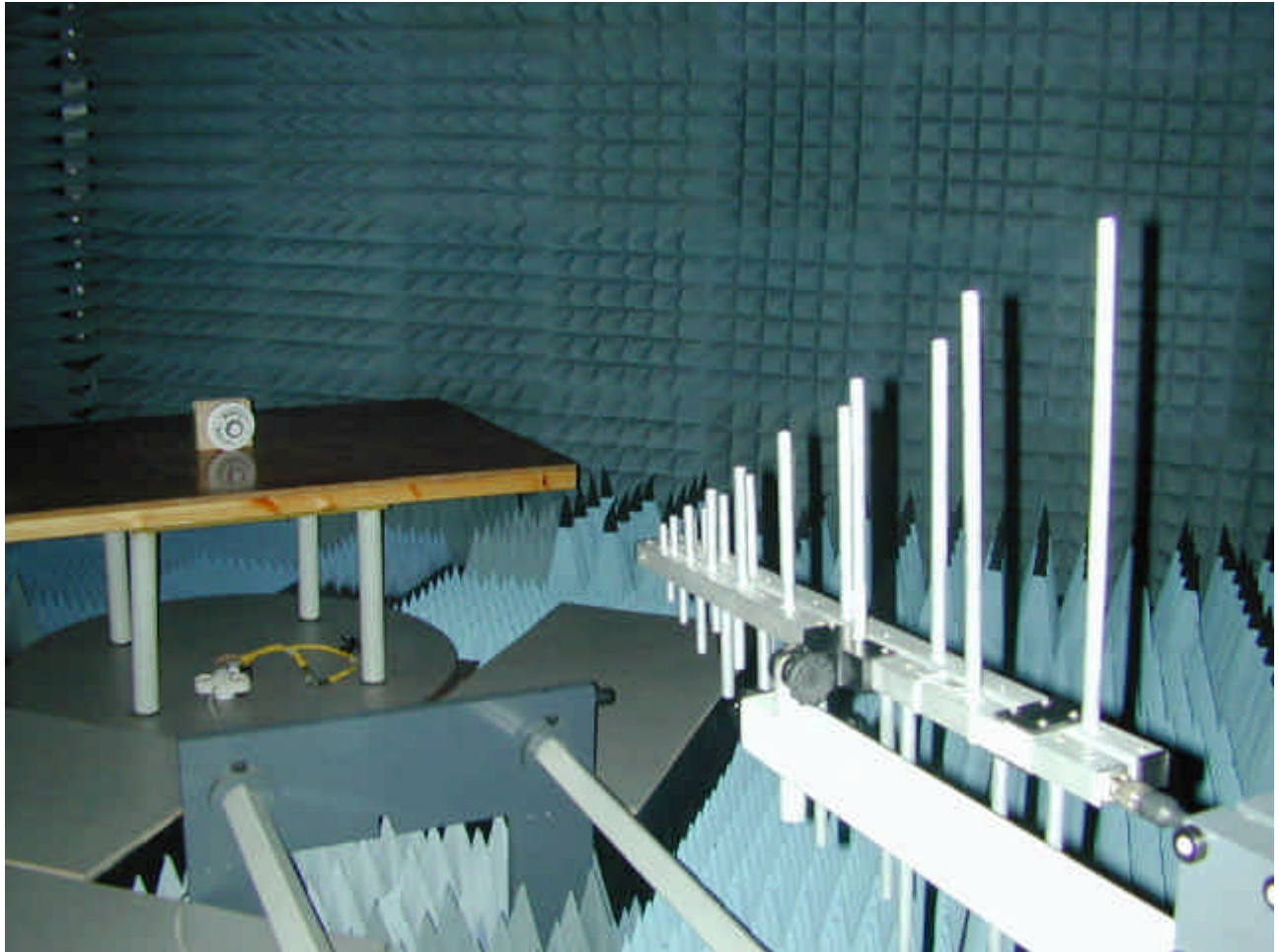
Photograph 3 Spurious emission measurement setup in 200 – 1000 MHz range, Log periodic antenna in vertical polarization
