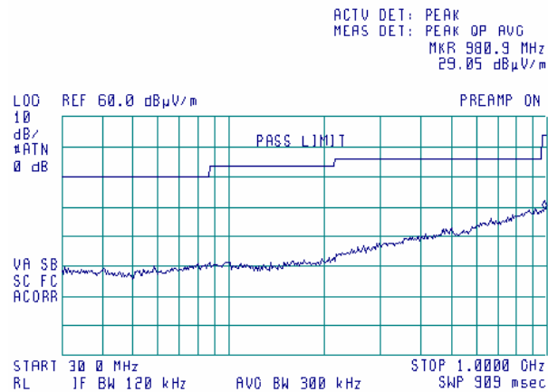
Plot 8.1.2 Radiated emission measurements in 30 - 1000 MHz range, vertical antenna polarization
