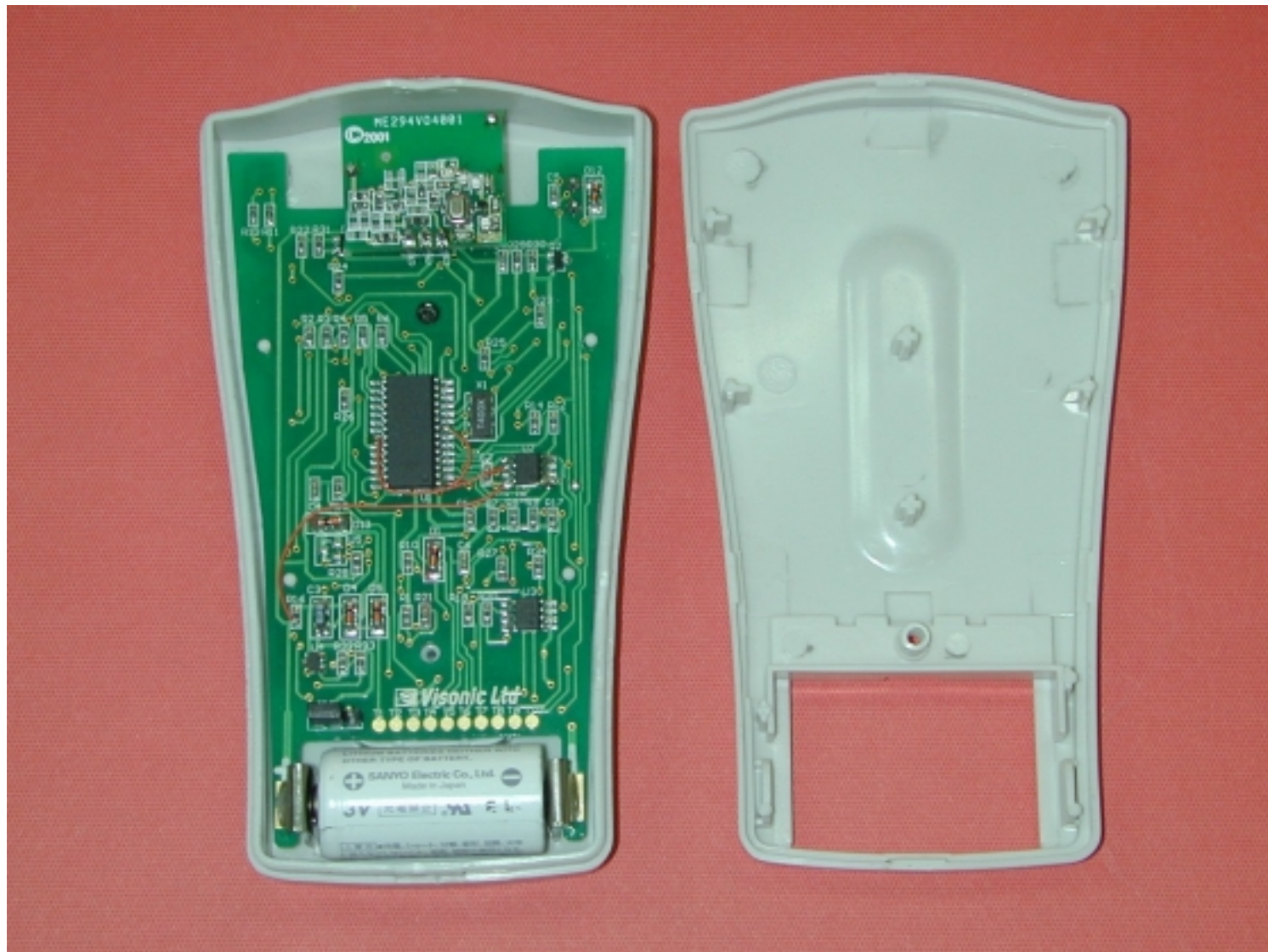
MCM140 internal view
