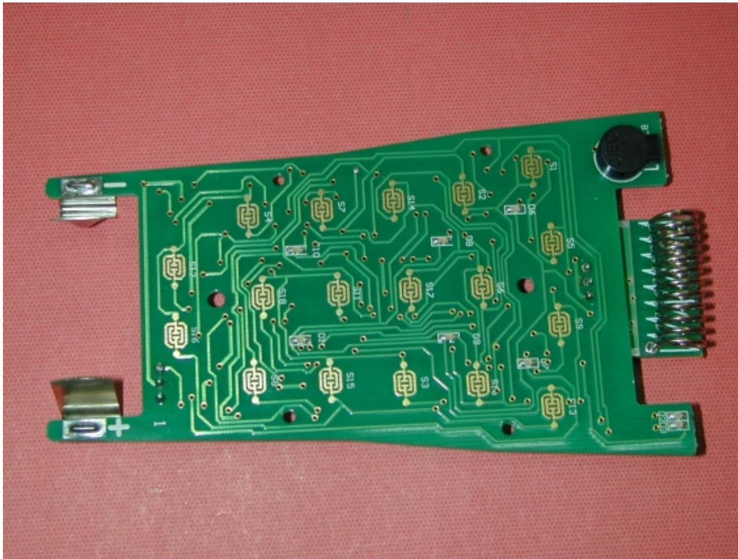
MCM140 PCB (second side)
