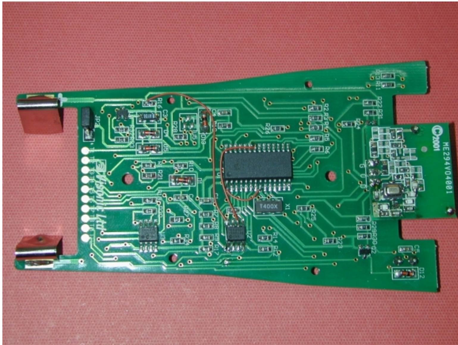
MCM140 PCB (first side)
