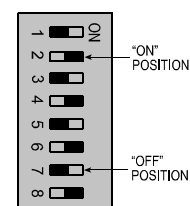
Figure 8. System Code Selector
