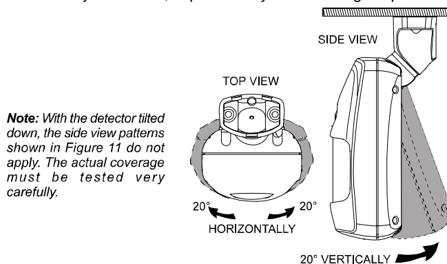
Figure 7. Tilt / Swivel Limits
