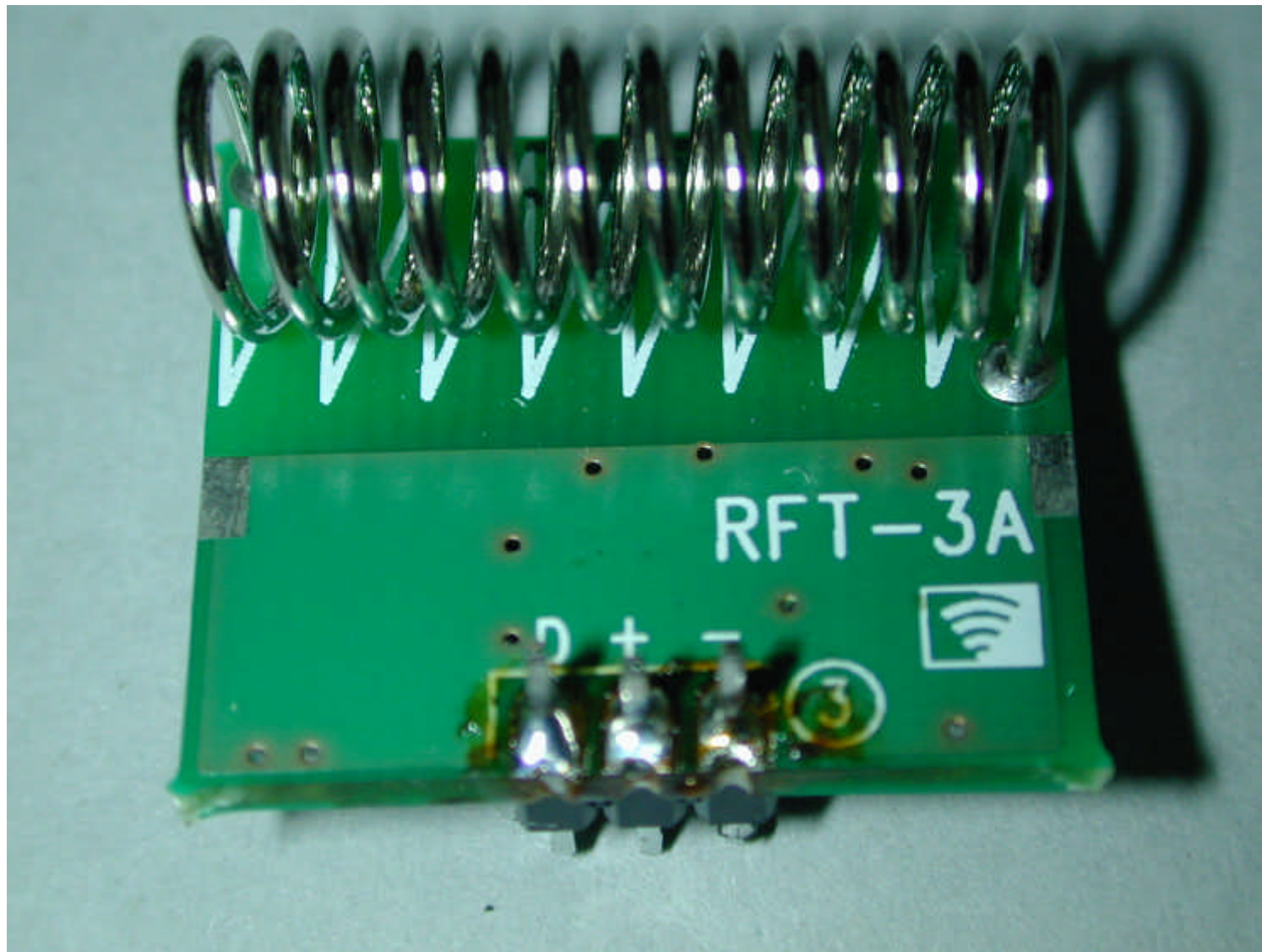
Transmitter module, first side
