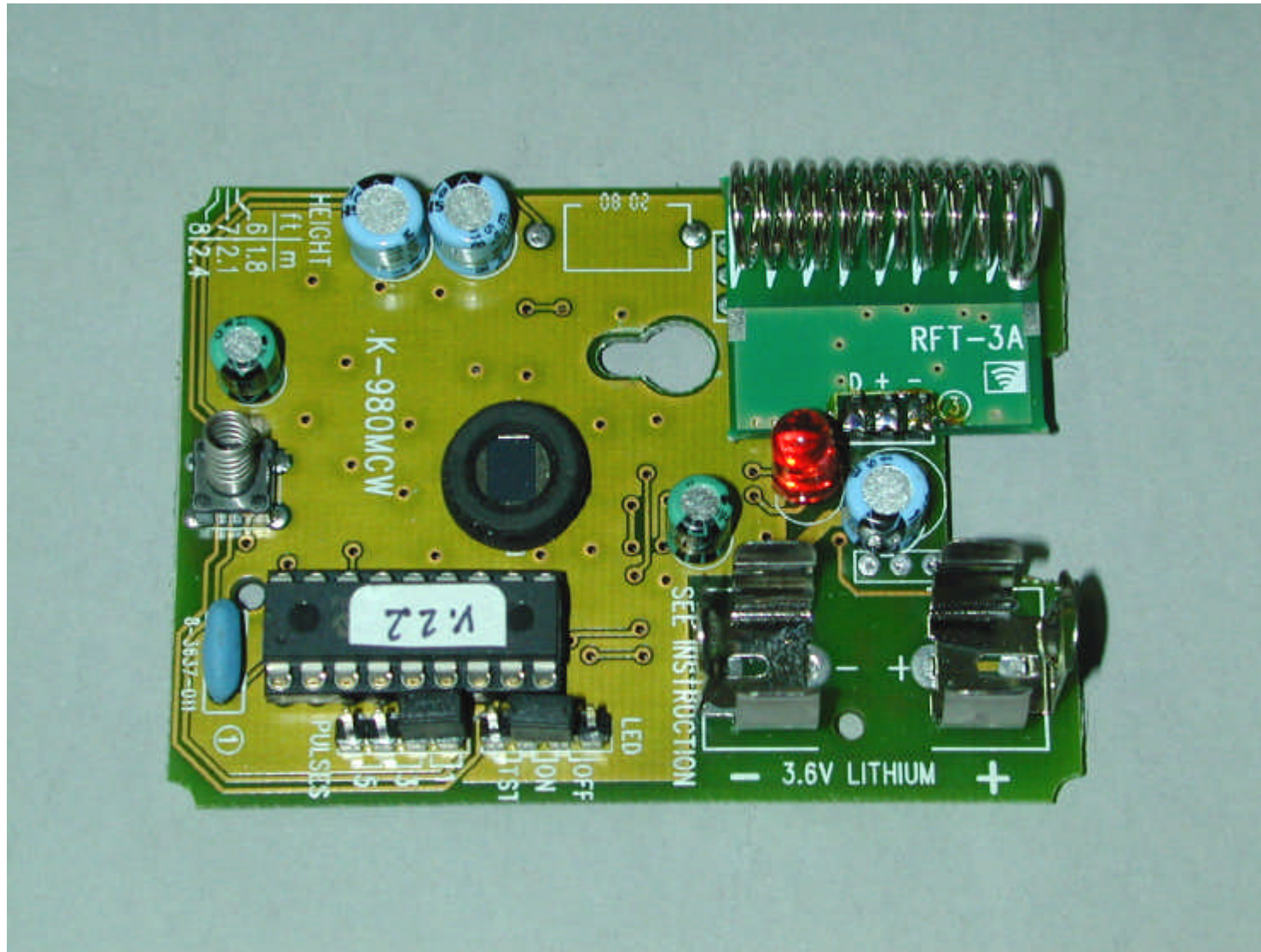
Internal view
