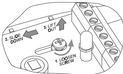
Figure 4. PCB Removal
