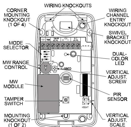
Figure 5. Inside View
