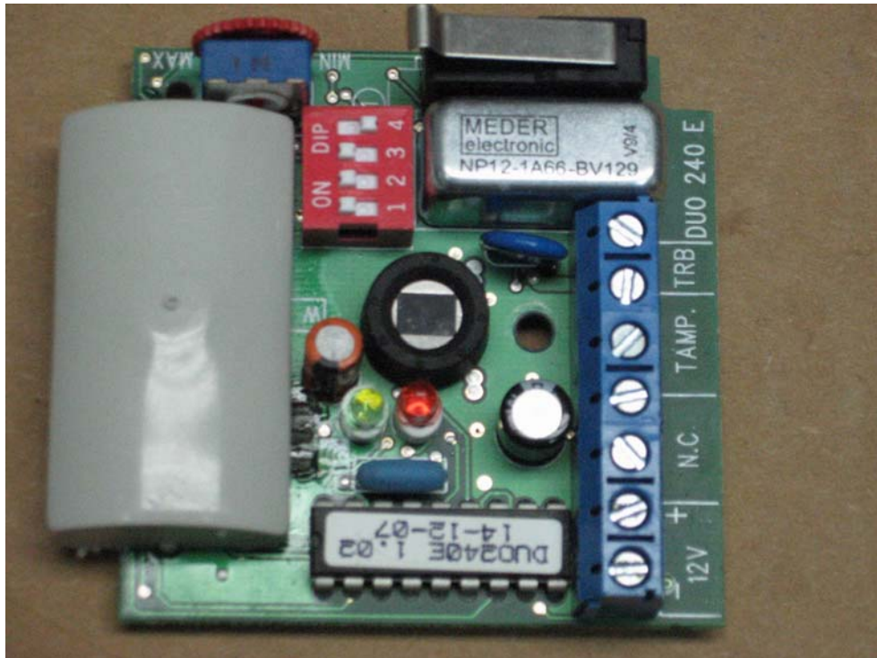
Figure 3: Top Side PCB
