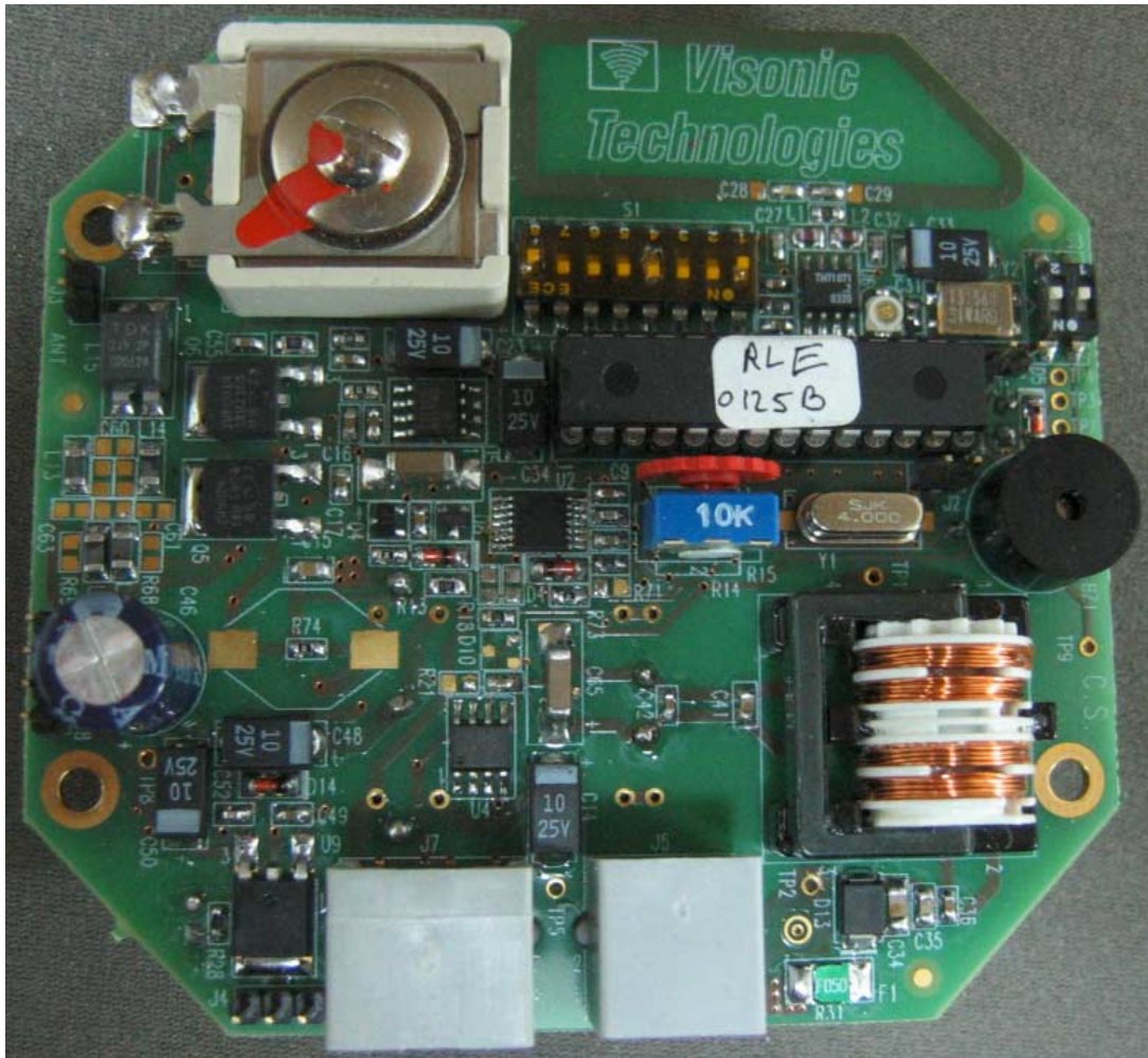
Photograph No.3 LF Exciter Component side of the PCB
