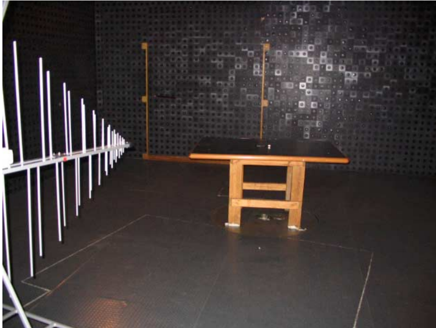
Photograph No.2 Setup for spurious emission field strength measurements in anechoic chamber above 30 MHz
