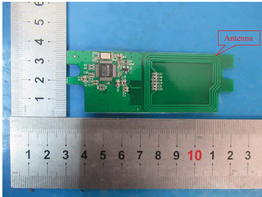
EUT – PCB-6 Chip View
